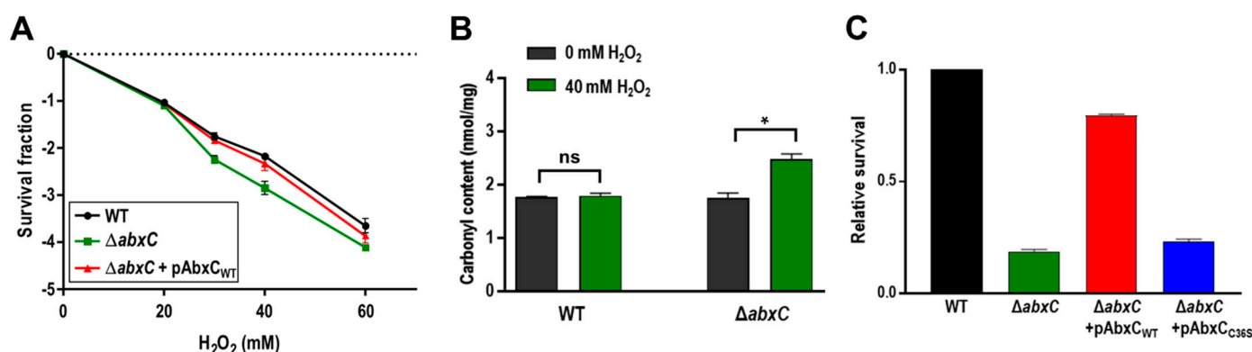
Figure 3. Effects of abxC mutation on H 2 O 2 resistance. (A) Survival of \Delta abxC exposed to H 2 O 2 . WT, \Delta abxC , and \Delta abxC harboring pAbxC WT that encodes the wild-type AbxC were treated with H 2 O 2 at the indicated concentrations for 1 h. The survival fraction was calculated by dividing the CFU of H 2 O 2 -treated cells by the CFU of non-treated cells. Values are means and standard deviations of two independent experiments conducted in duplicate. (B) Protein carbonylation of \Delta abxC in response to H 2 O 2 . After treatment of 40 mM H 2 O 2 for 1 h, the carbonylated protein contents of WT and \Delta abxC were measured by the 2,4-dinitrophenylhydrazine (DNPH) assay. Data represent the means \pm standard deviations of three independent experiments. Comparisons between two groups were performed by Student's t-test (GraphPad Prism 7.04). A p -value of less than 0.01 is considered statically significant (ns; not significant, *, p < 0.01). (C) Complementation of \Delta abxC . WT, \Delta abxC , and \Delta abxC harboring the pAbxC WT and pAbxC C36S plasmids, which produce the wild-type AbxC and its C36S mutant proteins, respectively, were treated with 40 mM H 2 O 2 for 1 h. Survival abilities of \Delta abxC mutants were expressed relative to WT survival (arbitrarily set at 1), i.e., the CFU of mutants were normalized to the CFU of WT. Data represent the means \pm standard deviations of three independent experiments.
