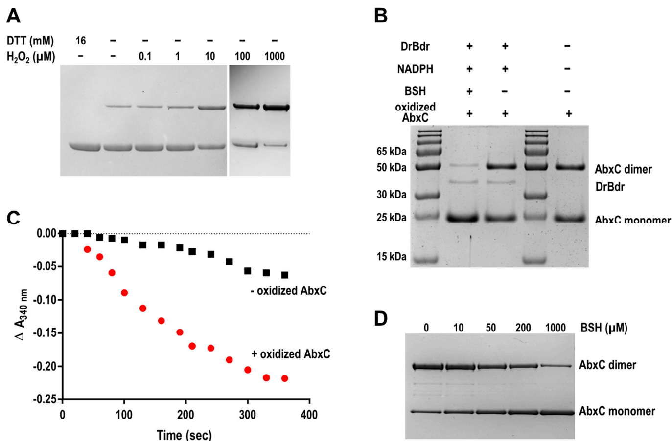
Figure 5. Dimer–monomer transition property of AbxC. (A) Effect of H 2 O 2 on AbxC oxidation. The purified AbxC proteins (0.5 mg/mL) were incubated with increasing concentrations of H 2 O 2 in PBS for 15 min and then separated using non-reducing SDS-PAGE (12% gels). DTT was used for AbxC reduction. (B) Effect of BSH in reduction of oxidized AbxC. AbxC proteins (0.5 mg/mL) oxidized by diamide treatment were incubated alone or with DrBdr (0.5 μM)/NADPH (500 μM)/BSH (500 μM) for 15 min in 20 mM Tris-HCl pH 7.5 at room temperature. The samples were analyzed by non-reducing SDS/PAGE. Bands representing the AbxC monomers and dimers and DrBdr are indicated. (C) NADPH consumption by oxidized AbxC. The reaction mixtures contained 500 μM BSH, 500 μM NADPH, and 0.5 μM DrBdr. Time-dependent consumption of NADPH was monitored at 340 nm immediately after addition of AbxC (– oxidized AbxC) or oxidized AbxC (+ oxidized AbxC). The experiments were repeated twice and representative data are shown. (D) Effect of BSH on AbxC reduction. AbxC proteins (0.5 mg/mL) were oxidized by diamide treatment and incubated with the indicated concentrations of BSH for 15 min in 20 mM Tris-HCl containing 500 μM NADPH. The mixtures were separated using non-reducing SDS-PAGE (12% gels).
