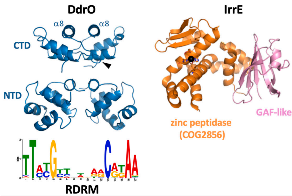
Figure 2. Crystal structures of DdrO and IrrE from D. deserti . For DdrO, the dimers of the C-terminal domain (CTD) and the DNA-binding N-terminal domain (NTD) are shown. The DdrO structure contains eight \alpha -helices (five in the NTD, three in the CTD), and IrrE cleaves DdrO in the loop connecting \alpha 7 and \alpha 8 (one cleavage site is indicated with an arrowhead). Sequence logo of the conserved radiation/desiccation motif (RDRM) to which DdrO binds is also shown.
