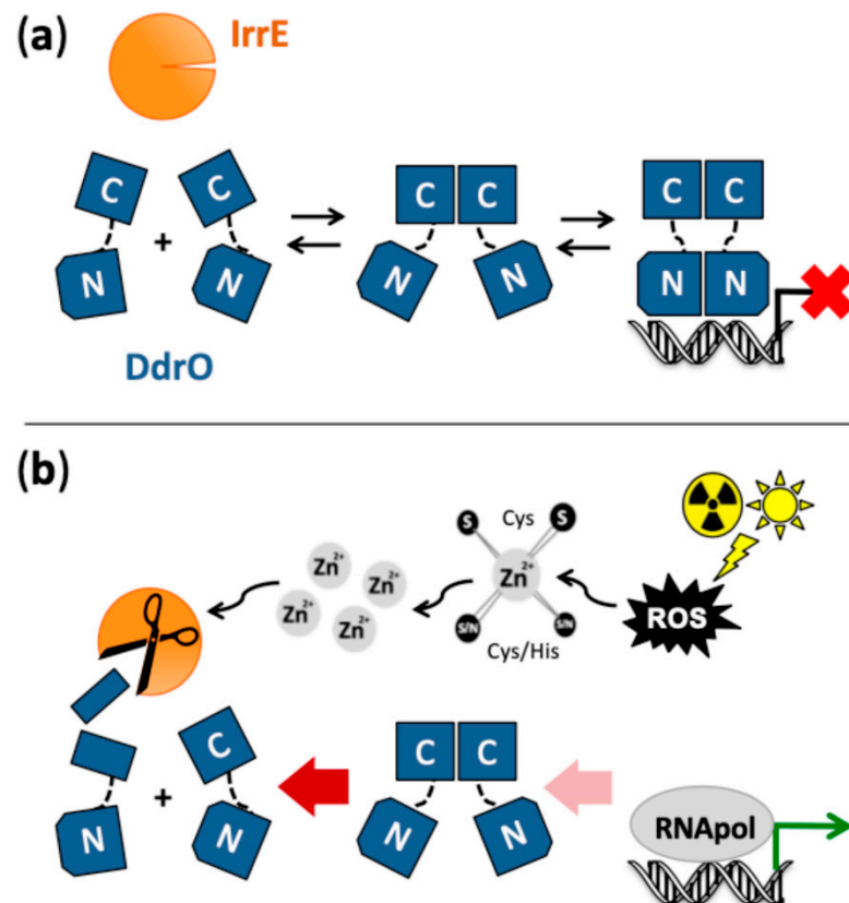
Figure 3. Proposed mechanism for induction of the SOS-independent radiation/desiccation response in Deinococcus . (a) Under standard conditions, the majority of zinc metalloproteinase IrrE is inactive due to limited availability of zinc ions, and repressor DdrO exists as a dynamic equilibrium between monomers and free and DNA-bound dimers. DdrO contains an N- and C-terminal domain separated by a flexible linker. DdrO dimerization is mediated by its C-terminal domain. Dimers of the N-terminal domain are expected mainly when DdrO is bound to the palindromic target DNA motif located in the promoter region of radiation/desiccation response (RDR) genes, which represses their transcription. (b) Exposure to conditions such as radiation and desiccation generates oxidative stress through formation of reactive oxygen species (ROS), which can cause oxidation of cysteine residues of zinc/cysteine sites in proteins, concomitantly causing release of zinc ions from these sites and a transient increase in the intracellular concentration of free, available zinc ions. The released zinc functions as second messenger, and increases the amount of active zinc-bound IrrE that cleaves the C-terminal domain of monomeric DdrO, abolishing its dimerization and shifting the DdrO equilibrium toward cleavable monomers. The diminished amount of DdrO leads to induced expression of the RDR regulon genes (including several DNA repair genes and ddrO itself). After the stress is alleviated and the zinc signal has disappeared, zinc availability for (newly synthesized) IrrE will become limited again, allowing DdrO to re-accumulate.
