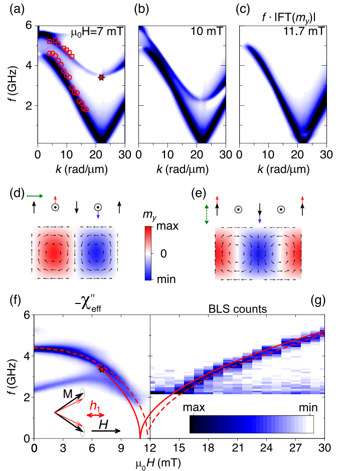
FIG. 3. (a)–(c) Color plot of the simulated spin-wave spectrum amplitude density as a function of wave vector and frequency, for a field of 7, 10, and 11.7 mT, respectively. In (a), the positions of the measured Brillouin light scattering peaks are reported as circles and squares and the Higgs mode frequency determined analytically is shown as a star. (d) Color plot of the distribution of the out-of-plane component of the dynamic magnetization for the Goldstone mode [ k = k_c , f = 0.1 GHz in (b)]. The vector plot shows the distribution of the transverse magnetization of the underlying static stripe modulation. (e) Same for the Higgs mode [ k = k_c , f = 3.5 GHz in (b)]. The green arrows sketch the motion of the stripe structure, namely a rigid displacement and an amplitude oscillation in (d) and (e), respectively. (f) Color plot of the microwave absorption measured in the stripe phase as a function of field and frequency, for the longitudinal pumping geometry sketched in the inset. (g) Color plot of the Brillouin light scattering intensity measured in the saturated phase as a function of field and frequency for a transferred wave vector k_c = 21 rad/ \mu\text{m} . The solid and dashed lines in (f) and (g) show the soft/Higgs mode frequency extracted from our analytical approach (see details in the Supplemental Material [24] and Ref. [41] therein) and from micromagnetic simulations, respectively. The (min, max) values for color plots are (4, 20) , (-1, -18) \times 10^{-3} , and (100, 300) for (a)–(c), (f), and (g), respectively.
