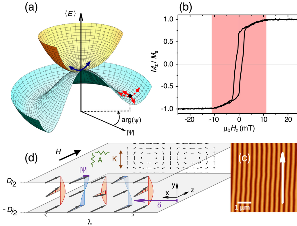
FIG. 1. (a) Sketch of the characteristic dynamic modes associated with U(1) symmetry breaking. The blue arrow shows the degenerate modes in the high-symmetry phase (yellow potential surface). The solid and dashed red arrows show the Goldstone and Higgs modes in the low-symmetry phase (sombbrero-shaped blue potential surface). (b) Magnetization loop measured for our 180-nm \text{Co}_{40}\text{Fe}_{40}\text{B}_{20} film with a magnetic field \mathbf{H} in the plane. (c) Magnetic force microscopy image of the weak stripe magnetic texture existing below the critical field H_c (shown here at remanence). The white arrow shows the direction of the previously applied field. (d) Sketch of the three-dimensional normalized magnetization distribution \mathbf{M}(x, y, z)/M_s within the weak stripe texture, together with its minimal description in terms of a U(1) symmetry breaking, with associated amplitude |\psi| and phase \arg(\psi) = k\delta (see details in the text).
