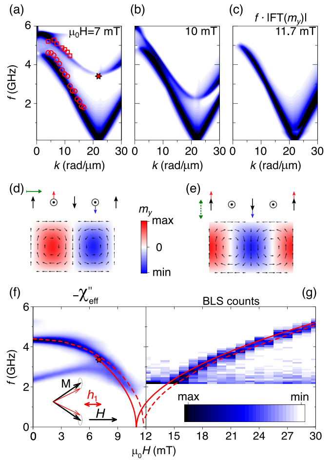
FIG. 3. (a)–(c) Color plot of the simulated spin-wave spectrum amplitude density as a function of wave vector and frequency, for a field of 7, 10, and 11.7 mT, respectively. In (a), the positions of the measured Brillouin light scattering peaks are reported as circles and squares and the Higgs mode frequency determined analytically is shown as a star. (d) Color plot of the distribution of the out-of-plane component of the dynamic magnetization for the Goldstone mode [ k = k_c , f = 0.1 GHz in (b)]. The vector plot shows the distribution of the transverse magnetization of the underlying static stripe modulation. (e) Same for the Higgs mode [ k = k_c , f = 3.5 GHz in (b)]. The green arrows sketch the motion of the stripe structure, namely a rigid displacement and an amplitude oscillation in (d) and (e), respectively. (f) Color plot of the microwave absorption measured in the stripe phase as a function of field and frequency, for the longitudinal pumping geometry sketched in the inset. (g) Color plot of the Brillouin light scattering intensity measured in the saturated phase as a function of field and frequency for a transferred wave vector k_c = 21 rad/ \mu\text{m} . The solid and dashed lines in (f) and (g) show the soft/Higgs mode frequency extracted from our analytical approach (see details in the Supplemental Material [24] and Ref. [41] therein) and from micromagnetic simulations, respectively. The (min, max) values for color plots are (4, 20) , (-1, -18) \times 10^{-3} , and (100, 300) for (a)–(c), (f), and (g), respectively.
