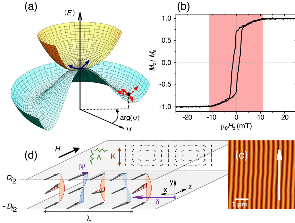
FIG. 1. (a) Sketch of the characteristic dynamic modes associated with U(1) symmetry breaking. The blue arrow shows the degenerate modes in the high-symmetry phase (yellow potential surface). The solid and dashed red arrows show the Goldstone and Higgs modes in the low-symmetry phase (sombbrero-shaped blue potential surface). (b) Magnetization loop measured for our 180-nm \text{Co}_{40}\text{Fe}_{40}\text{B}_{20} film with a magnetic field \mathbf{H} in the plane. (c) Magnetic force microscopy image of the weak stripe magnetic texture existing below the critical field H_c (shown here at remanence). The white arrow shows the direction of the previously applied field. (d) Sketch of the three-dimensional normalized magnetization distribution \mathbf{M}(x, y, z)/M_s within the weak stripe texture, together with its minimal description in terms of a U(1) symmetry breaking, with associated amplitude |\psi| and phase \arg(\psi) = k\delta (see details in the text).
