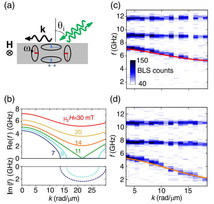
FIG. 2. (a) Sketch of the Damon-Eshbach geometry, magnetization precession (black ellipses), and basis functions used for modeling (red and blue bars). The thin bars can be combined to form the stray-field-free ansatz of Eq. (1), while the thick bars, orthogonal to them, carry nonzero magnetic pseudocharges, as shown at the bottom of the film. (b) Spin-wave dispersion relations calculated analytically using the basis of (a) (see details in the text and Refs. [24,31–33]), for an external field of 30, 20, 14, 11, 9, and 7 mT. For the last two values, the saturated state is unstable, and the spin-wave frequency becomes imaginary over a certain range of wave numbers (see the distinct vertical scale at the bottom of the graph). (c), (d) Color maps of the Brillouin light scattering intensity measured as function of the transferred wave vector [scattering geometry shown by the green arrows in (a)] and transferred frequency f under an external field of \mu_0 H = 30 and 14 mT, respectively. The lines show the calculated soft mode frequency [same as in (b)].
