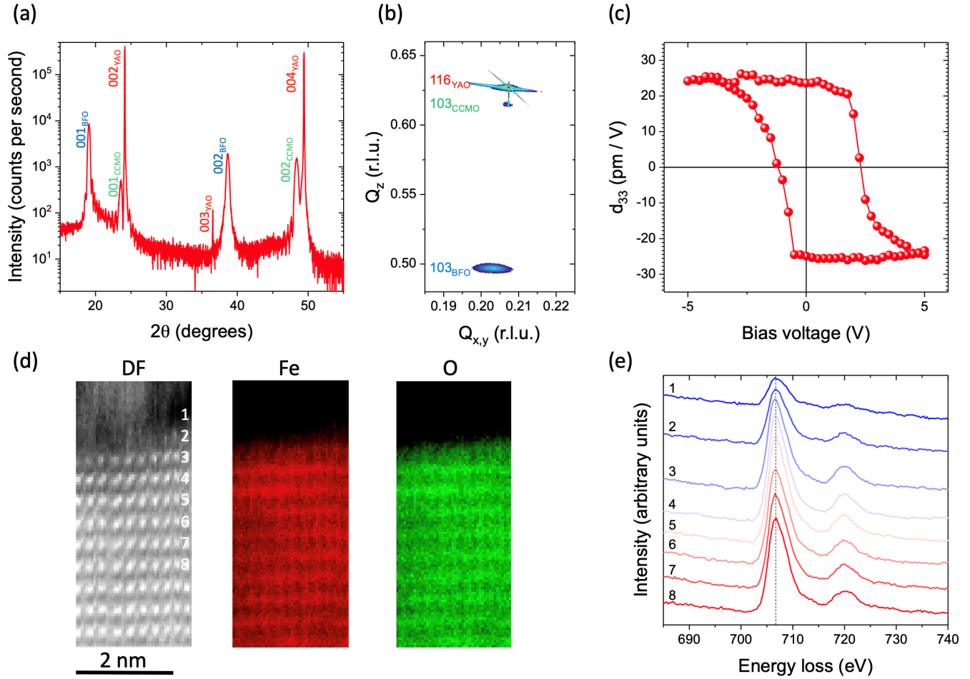
FIG. 1. (a) 2\theta -x-ray diffraction scan of a \text{BiFeO}_3 thin film on \text{Ca}_{0.96}\text{Ce}_{0.04}\text{MnO}_3/\text{YAlO}_3 (001). (b) Reciprocal space mapping around the \text{YAlO}_3 (116) peak. These structural characterizations indicate that \text{BiFeO}_3 is only in its super-tetragonal phase. (c) Local piezoelectric loop as a function of the bias voltage applied to the \text{Ca}_{0.96}\text{Ce}_{0.04}\text{MnO}_3 electrode. The imprint to the right indicates a preferential downward polarization orientation. (d) Dark-field (DF) and electron energy loss spectroscopy images at the Fe and O edges. (e) Spectra at the Fe L edge showing that the Fe valence is not modified at the surface. BFO, \text{BiFeO}_3 ; CCMO, \text{Ca}_{0.96}\text{Ce}_{0.04}\text{MnO}_3 ; r.l.u., reciprocal lattice units; YAO, \text{YAlO}_3 .
