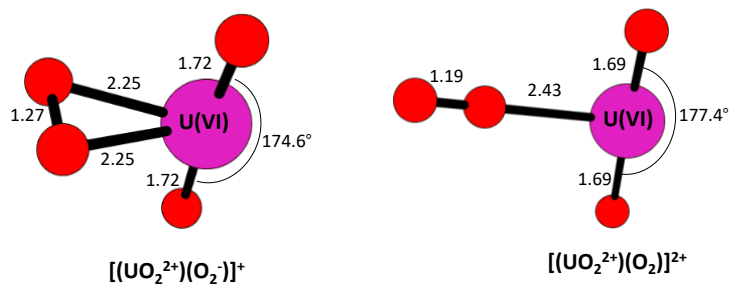
Figure 8. Computed structures for O 2 addition to uranyl(V) and uranyl(VI) to yield uranyl(VI). Left: Superoxide [(\text{UO}_2^{2+})(\text{O}_2^-)]^+ from addition to \text{UO}_2^{2+} ; Right: Adduct [(\text{UO}_2^{2+})(\text{O}_2)]^{2+} from addition to \text{UO}_2^{2+} . Bond distances are in Å; O y1 -U-O y1 angles are in degrees. The corresponding U-O y1 distances are 1.74 Å for bare \text{U}^{\text{V}}\text{O}_2^+ and 1.68 Å for bare \text{U}^{\text{VI}}\text{O}_2^{2+} .
