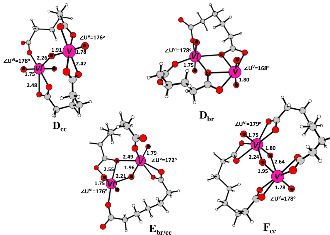
Figure 6. Computed structures D_{cc} and D_{br} for species [(UO_2^+)(UO_2^{2+})(C6^{2-})_2]^- ; E_{br/cc} for [(UO_2^+)(UO_2^{2+})(C7^{2-})_2]^- ; and F_{cc} for [(UO_2^+)(UO_2^{2+})(C8^{2-})_2]^- . Pink = U; red = O; grey = C; light grey = H. Uranyl O_{yl} are identified by black dots, and bridging O atoms by “br”. U oxidation states +V or +VI are indicated. Selected bond distances are given in Å. Uranyl angles \angle[O_{yl}-U^{VI}-O_{yl}] ( \angle U^{VI} ) and \angle[O_{yl}-U^V-O_{yl}] ( \angle U^V ) are in degrees.
