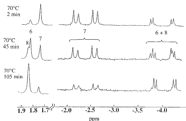
Figure 3. Representative ^1\text{H} -NMR spectra for the thermal treatment of a mixture of compounds 6 and 7 in \text{CD}_3\text{CN} . The different regions of the spectra are on different vertical scales.
