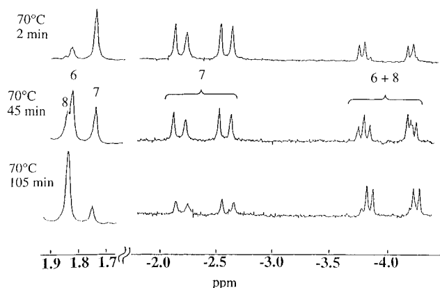
Figure 3. Representative ^1\text{H} -NMR spectra for the thermal treatment of a mixture of compounds 6 and 7 in \text{CD}_3\text{CN} . The different regions of the spectra are on different vertical scales.
