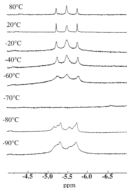
Figure 2. Temperature dependence of the ^1\text{H} -NMR hydride resonance of compound 5 . The solvent is \text{CD}_3\text{CN} for the spectra at 80 and 20 °C and \text{CD}_2\text{Cl}_2 for all the other spectra.
