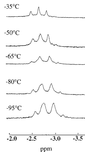
Figure 1. Variable-temperature ^1\text{H} -NMR spectrum of compound 4 in \text{CDFCl}_2 .
