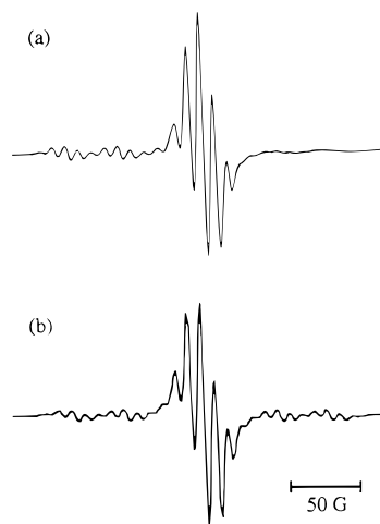
Figure 1. Experimental (a) and simulated (b) spectrum for complex [ 2 ] + . Solvent = acetone.
