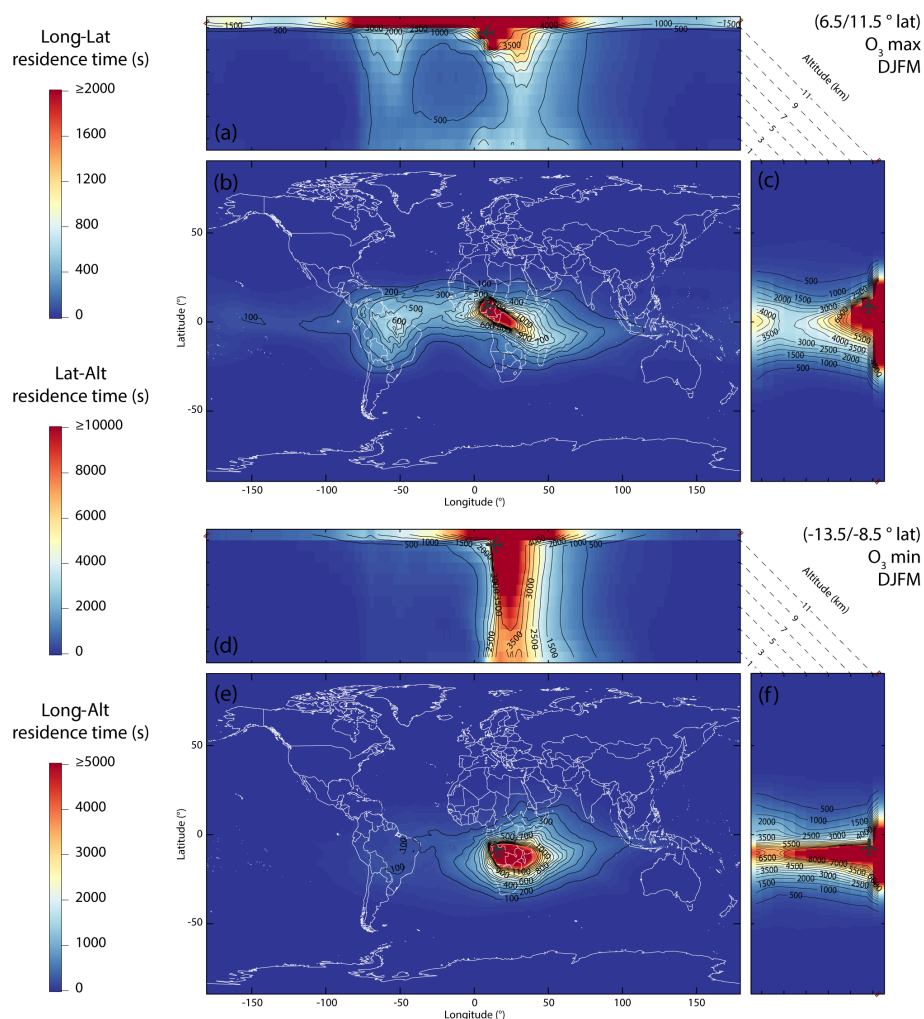
Figure 7. FLEXPART backward plume of air masses where IAGOS flights have recorded maxima (between 6.5 and 11.5° N: a, b, c ) and minima (between 13.5 and 8.5° S: d, e, f ) of ozone in DJFM. Plumes are represented in terms of the residence time of particles in each individual output box in seconds, summed on the 20 d backward, on 5° lat of flight and on total column (latitude column for a, d , altitude column for b, e , and longitude column for c, f ), and averaged over all studied years. Note that the color scale is different for longitude–altitude profiles ( a, d ), longitude–latitude maps ( b, e ) and latitude–altitude profiles ( c, f ).
