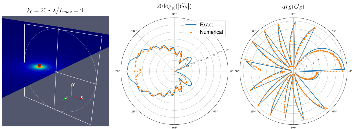
Figure 7: Relative Green's function G_S(\mathbf{x}, \mathbf{y}) for a semi-infinite plate for the fixed source at \mathbf{y} = (-1.0\text{ m}, 0.1\text{ m}, 0) and a varying observation point on the circle of radius r_x = 2\text{ m} in the plane x_3 = 0 . Comparison between the numerical and analytical solutions for the wave number k_0 = 20\text{ m}^{-1} .
