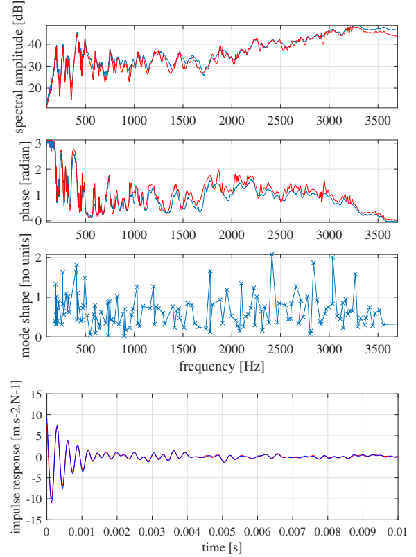
FIG. 4. (color online) Bridge and soundboard modal analysis. Top panel: comparison of the spectral magnitude (Ref 1 dB : 1 m.s ^{-2} .N ^{-1} ) of the measured (blue ) and reconstructed (red ) FRF. Second panel, corresponding unwrapped phase), third panel corresponding mode shapes. Bottom panel: corresponding measured (blue) and reconstructed (red) impulse responses.
