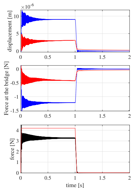
FIG. 13. (color online) Bottom: force applied on the key and resulting force on the tangent. Middle: force on the bridge with (red) and without (blue) dampers. Top: bridge displacement with (red) and without (blue) dampers.
