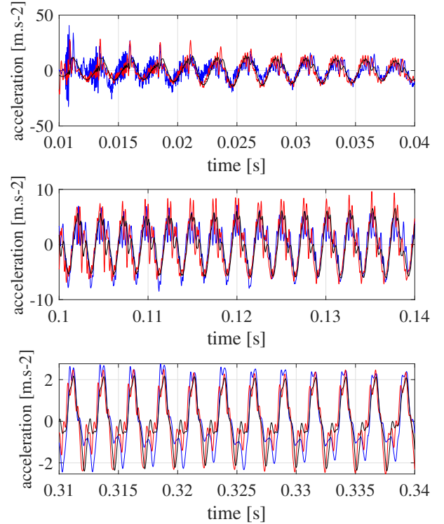
FIG. 12. Bridge acceleration waveforms at different times. Measurement in blue, simulation (3500 Hz modal truncation) in red, simulation (600 Hz modal truncation) in black.
