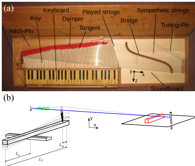
FIG. 1. (color online) (a) Description of a clavichord and (b) Sketch of the clavichord's mechanism in three positions of the touch: at rest, the tangent flushing the string and after excitation
