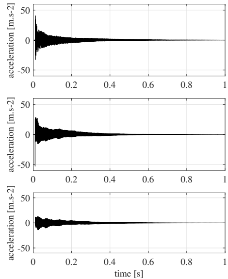
FIG. 11. (color online) Bridge acceleration waveforms (1s). Top: measurement. Middle: simulation (3500 Hz modal truncation). Bottom: simulation (600 Hz modal truncation).
