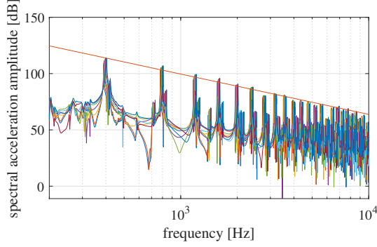
FIG. 10. (color online) Logarithmic spectral magnitude of bridge acceleration (ref 1 dB : 1 m.s -2 ), for different impact velocity of the key-tangent subsystem, with the average spectral slope.
