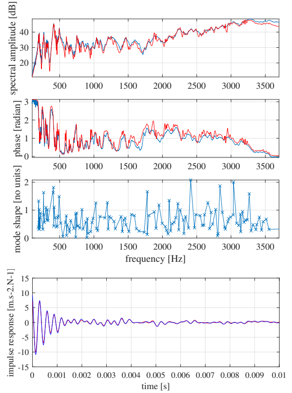
FIG. 4. (color online) Bridge and soundboard modal analysis. Top panel: comparison of the spectral magnitude (Ref 1 dB : 1 m.s -2 .N -1 ) of the measured (blue ) and reconstructed (red ) FRF. Second panel, corresponding unwrapped phase), third panel corresponding mode shapes. Bottom panel: corresponding measured (blue) and reconstructed (red) impulse responses.
