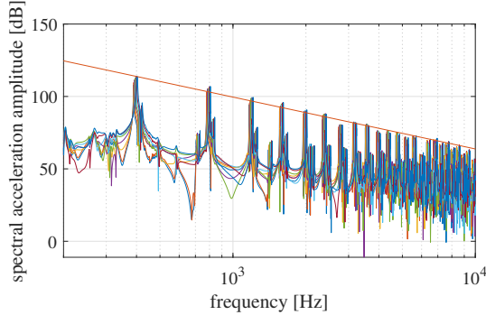
FIG. 10. (color online) Logarithmic spectral magnitude of bridge acceleration (ref 1 dB : 1 \text{ m.s}^{-2} ), for different impact velocity of the key-tangent subsystem, with the average spectral slope.
