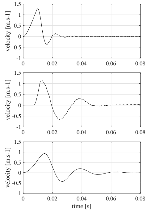
FIG. 7. Comparison of simulated and measured velocity at the tangent-string contact point. Top panel: "light key" simulation; middle panel: measurement; bottom panel: "heavy key" simulation.
