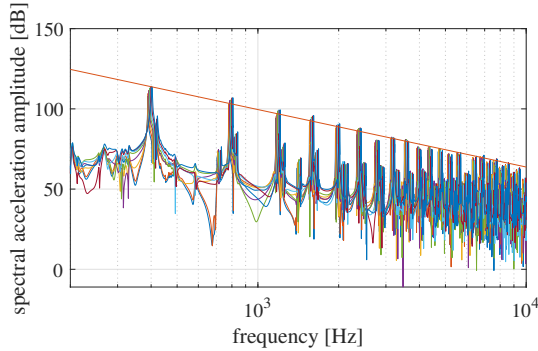
FIG. 10. (color online) Logarithmic spectral magnitude of bridge acceleration (ref 1 dB : 1 m.s -2 ), for different impact velocity of the key-tangent subsystem), with the average spectral slope.
