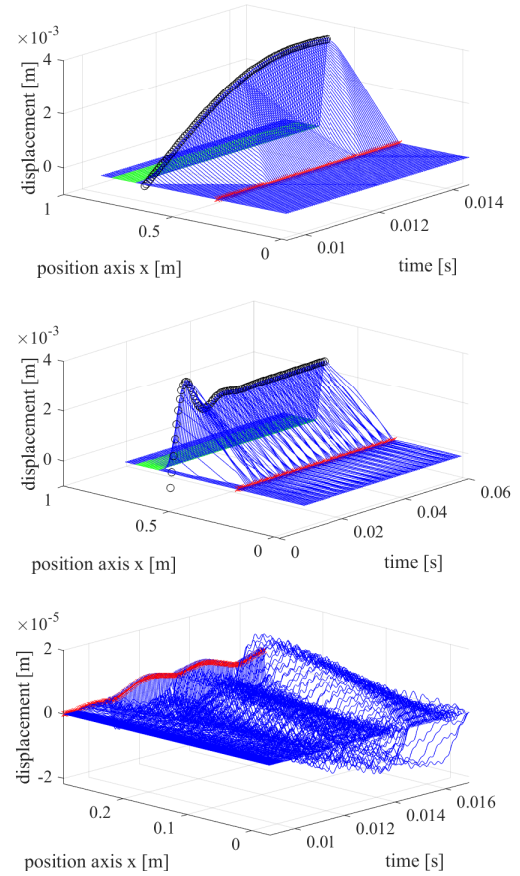
FIG. 6. (color online) History of the transverse motion for the G# 3 string. x axis: time (s); y axis : string length; z axis: transverse string motion. Top panel: full string between t = 10.0 ms and t = 14.0 ms. Middle panel: full string between t = 7.0 ms and t = 57.0 ms. Bottom panel: sympathetic part alone, between t = 9.0 ms and t = 17.0 ms.
