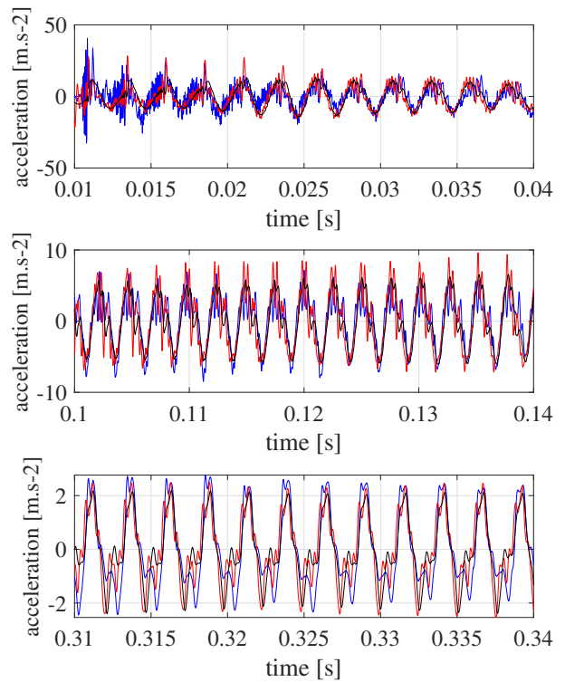
FIG. 12. Bridge acceleration waveforms at different times. Measurement in blue, simulation (3500 Hz modal truncation) in red, simulation (600 Hz modal truncation) in black.
