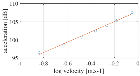
FIG. 9. (color online) Logarithmic bridge acceleration (ref 1 dB : 1 m.s -2 ) as a function of the logarithmic tangent impact velocity.
