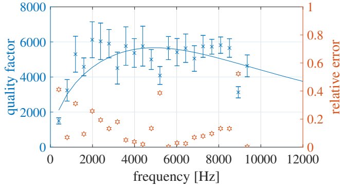
FIG. 3. (color online) String quality factor: experimental (blue cross) and theoretical (blue line, 95 % error bars (blue bar) and relative error (red star).
