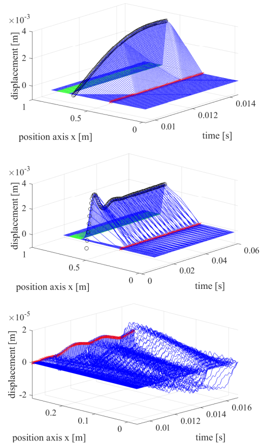
FIG. 6. (color online) History of the transverse motion for the G# 3 string. x axis: time (s); y axis: string length; z axis: transverse string motion. Top panel: full string between t = 10.0 ms and t = 14.0 ms. Middle panel: full string between t = 7.0 ms and t = 57.0 ms. Bottom panel: sympathetic part alone, between t = 9.0 ms and t = 17.0 ms.
