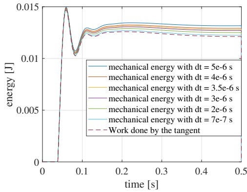
FIG. 5. (color online) Convergence of the total mechanical energy of the system compared to the work done by the tangent.
