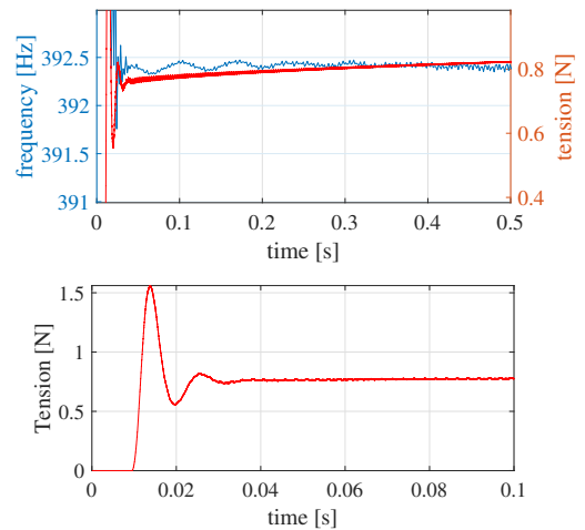
FIG. 8. (color online) Top: Dynamic tension of the string (red) and corresponding fundamental frequency (blue) for a 0.5 s note. Bottom: zoom of this same dynamic tension of the string in the first 0.1 s.
