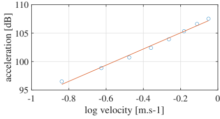
FIG. 9. (color online) Logarithmic bridge acceleration (ref 1 dB : 1 \text{ m.s}^{-2} ) as a function of the logarithmic tangent impact velocity.
