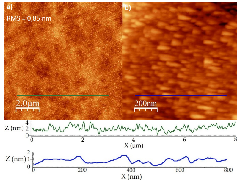
Figure 5. 10 \mu\text{m} \times 10 \mu\text{m} (a) and 1 \mu\text{m} \times 1 \mu\text{m} (b) AFM image of the GaP/Si sample. The green and blue lines show the profiles in both scans.
