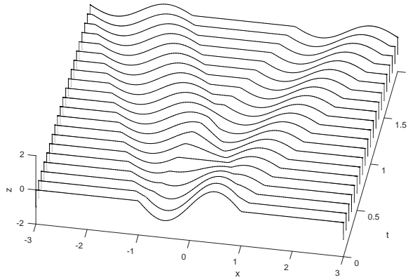
Fig. 1 Free evolution of the linear wave equation.
