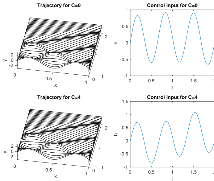
Fig. 2 Control of the nonlinear wave equation: f(u) = Cu^2 .
