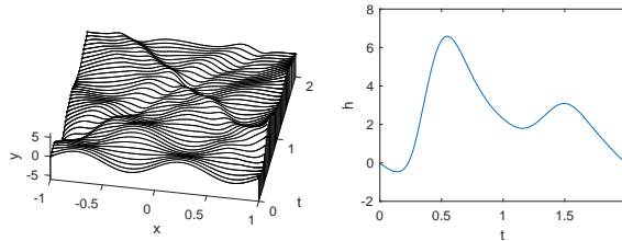
Fig. 4 Control of the semilinear wave equation: f(u) = -4u^3 .
