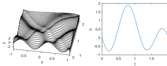
Fig. 5 Control of the semilinear wave equation: f(u) = 6 \sin u .
