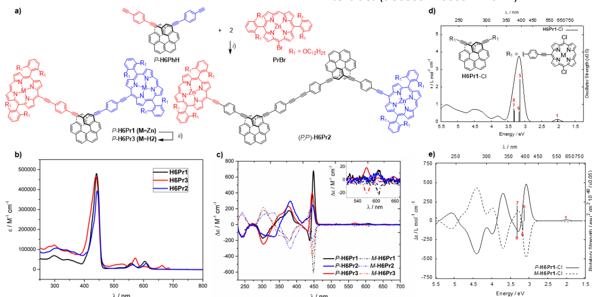
Figure 1. a) Synthetic pathway to H6Pr1 , H6Pr2 and H6Pr3 . i) \text{Pd}(\text{PPh}_3)_4 , \text{CuI} , Toluene/ \text{Et}_3\text{N} ; ii) TFA, DCM, TLC monitoring. Experimental b) UV-vis and c) ECD spectra of helicene-porphyrin conjugates H6Pr1 , H6Pr2 and H6Pr3 , d) chemical structure of the calculated model H6Pr1-Cl and calculated UV-vis spectrum e) calculated mirror-image ECD spectra.
