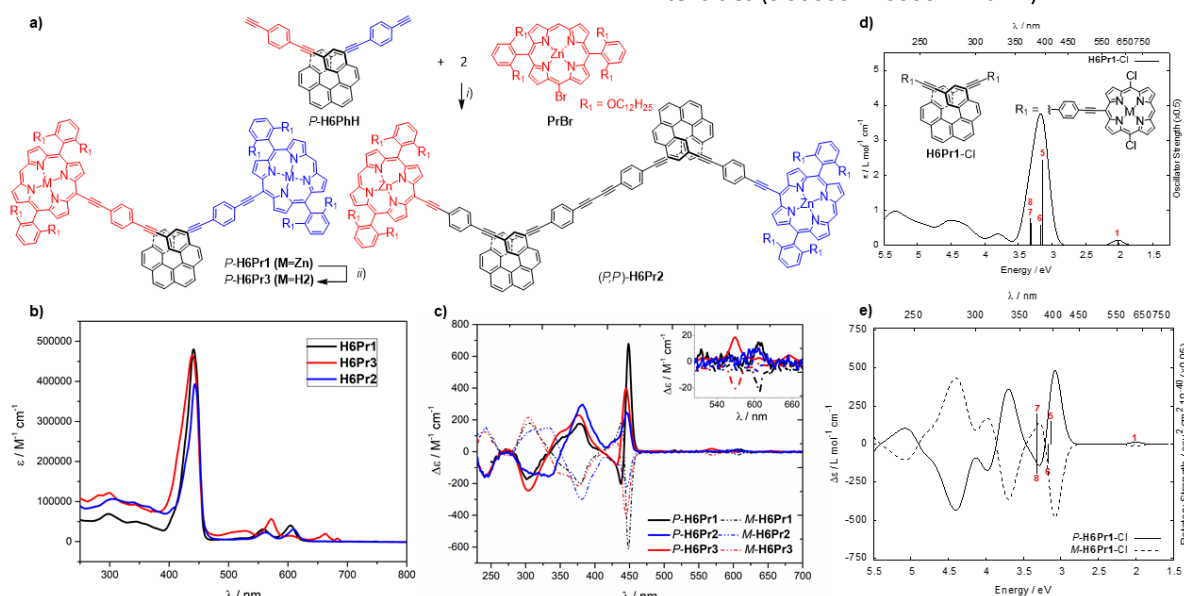
Figure 1. a) Synthetic pathway to H6Pr1 , H6Pr2 and H6Pr3 . i) \text{Pd}(\text{PPh}_3)_2 , \text{CuI} , Toluene/ \text{Et}_3\text{N} ; ii) TFA, DCM, TLC monitoring. Experimental b) UV-vis and c) ECD spectra of helicene-porphyrin conjugates H6Pr1 , H6Pr2 and H6Pr3 , d) chemical structure of the calculated model H6Pr1-Cl and calculated UV-vis spectrum e) calculated mirror-image ECD spectra.
