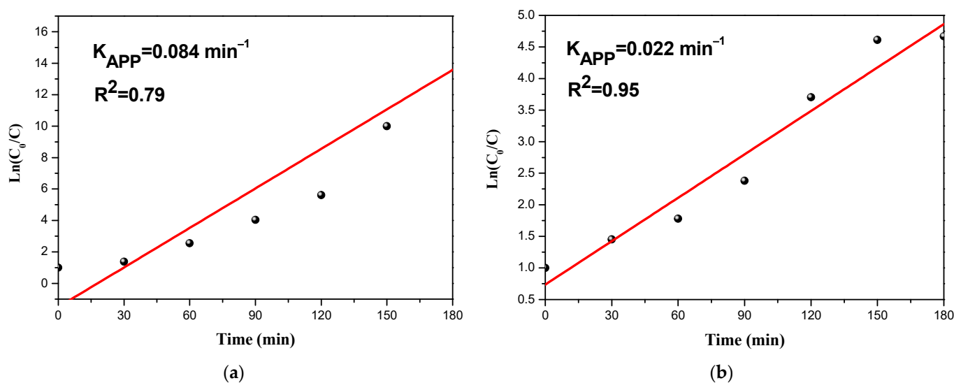
Figure 9. Pseudo-first-order kinetic plot (a) of the CFX degradation (b) of Cr(VI) reduction.
