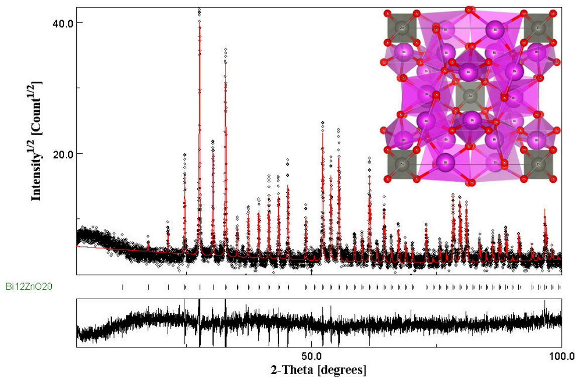
Figure 2. Rietveld refined XRD pattern for the \text{Bi}_{12}\text{ZnO}_{20} nanoparticles. The circles represent experimental points and the red line represents Rietveld refined data. Inset: supercell model for bulk \text{Bi}_{12}\text{ZnO}_{20} .
