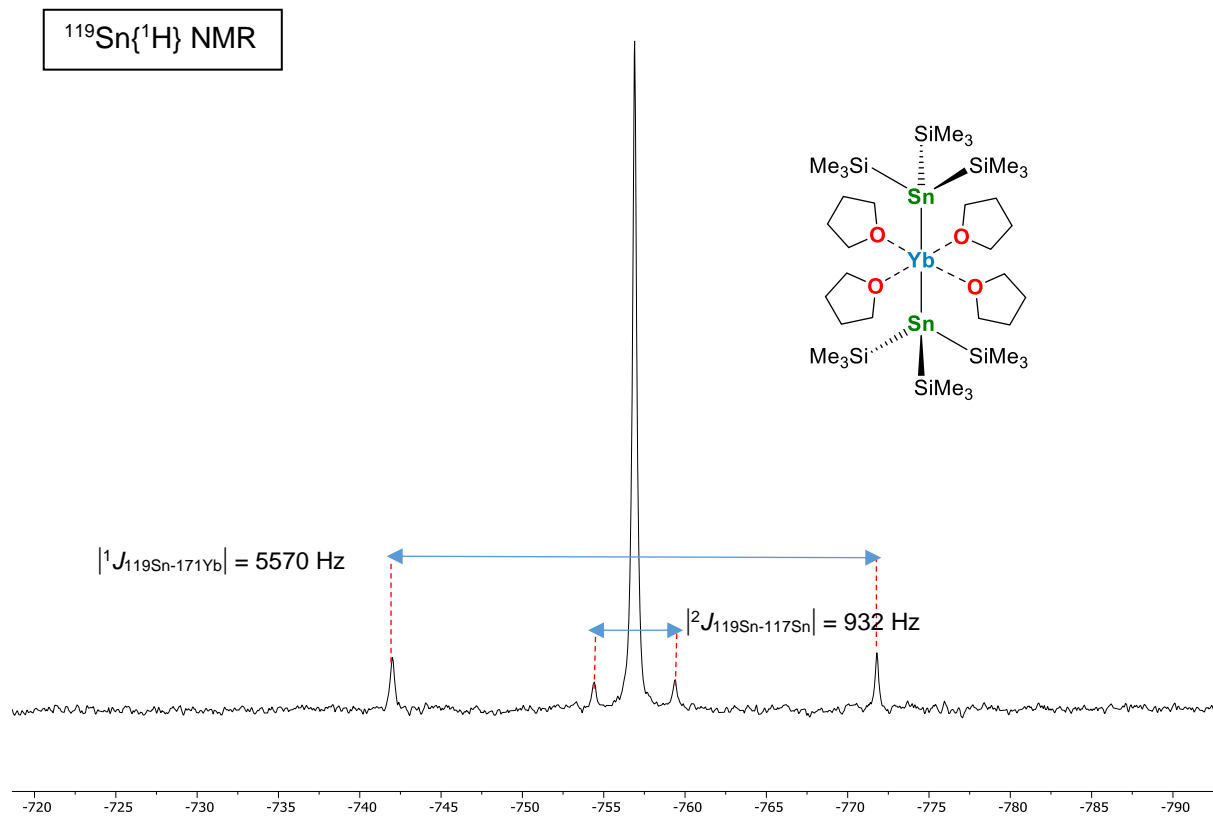
Figure 3. ^{119}\text{Sn}\{^1\text{H}\} NMR spectrum (186.36 MHz, benzene- d_6 , 300 K) of [\text{Yb}\{\text{Sn}(\text{SiMe}_3)_3\}_2\cdot(\text{thf})_4] ( Yb-Sn ).
