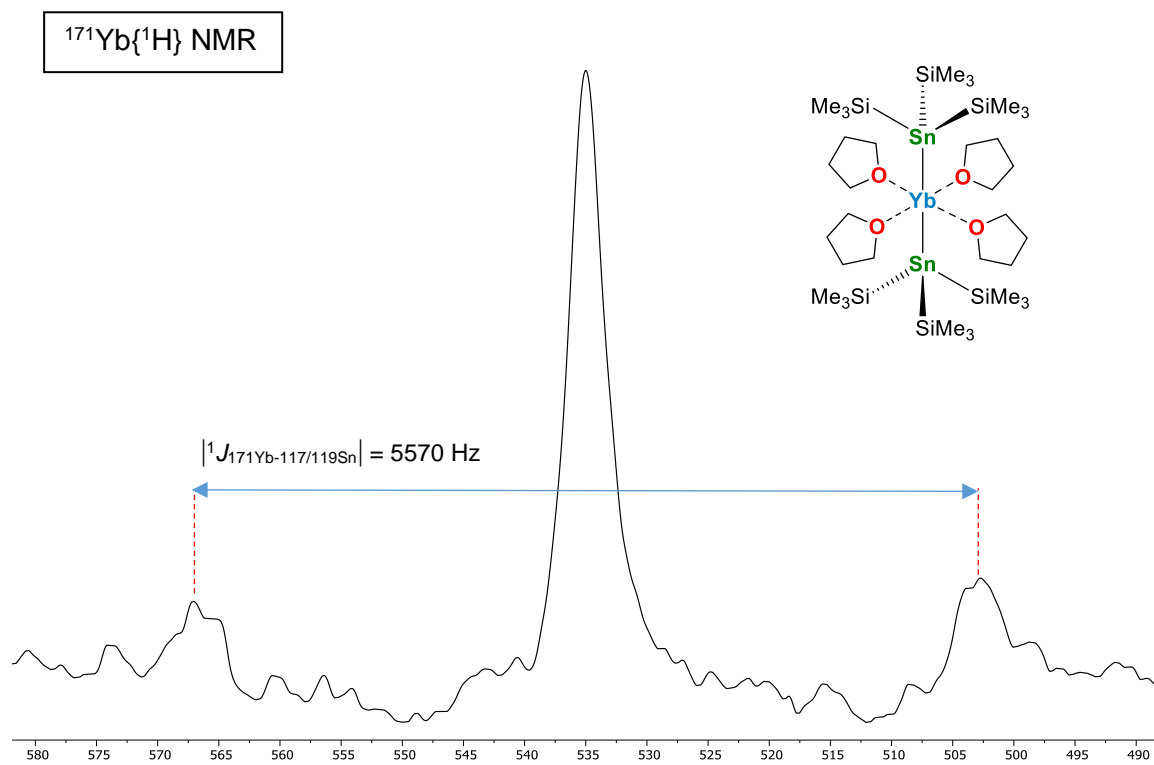
Figure 4. ^{171}\text{Yb}\{^1\text{H}\} NMR spectrum (87.57 MHz, benzene- d_6 , 300 K) of [\text{Yb}\{\text{Sn}(\text{SiMe}_3)_3\}_2\cdot(\text{thf})_4] ( Yb-Sn ).
