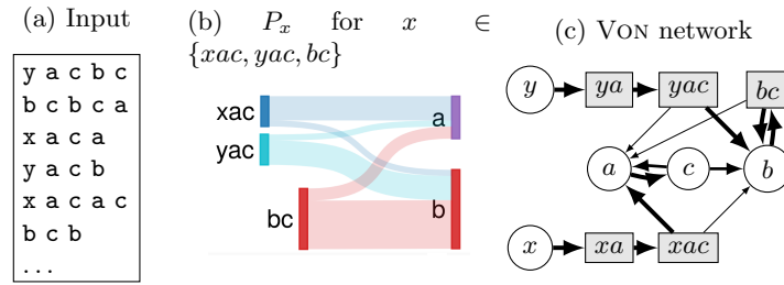
Fig. 1: Example of inputs and variable-order networks representing dependencies between items \Omega = \{x, y, a, b, c\} . We can identify 2nd or 3rd order dependencies in (b). For instance, when visiting x then a then c , the flow tends to return to a . The VON( \mathcal{S} ) network in (c) only includes relevant dependencies. Subsequence ac is not a relevant extension of the sequence c since knowing we visited a before c does not impact the prediction of the next visited item. Memory-nodes are displayed as grey rectangles. The set \mathcal{V}(c) = \{xac, yac, bc, c\} are representations of item c .
