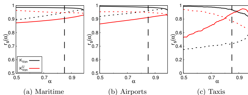
Fig. 5: Evolution of the Spearman correlation coefficient r_s(\alpha) with \alpha , for couples of rankings. Solid lines (dashed lines) are related to correlations with Biased 1 st ONPR (1 st ONPR U ). Vertical black dashed line represents \alpha = 0.85 .
