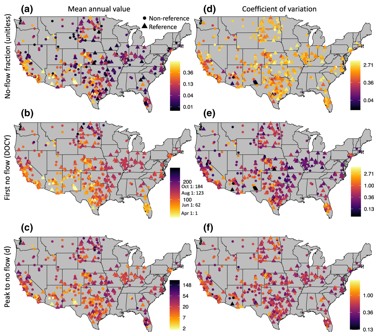
Figure 2. Spatial distribution of mean annual no-flow metrics (a–c) and their coefficients of variation (d–f).
