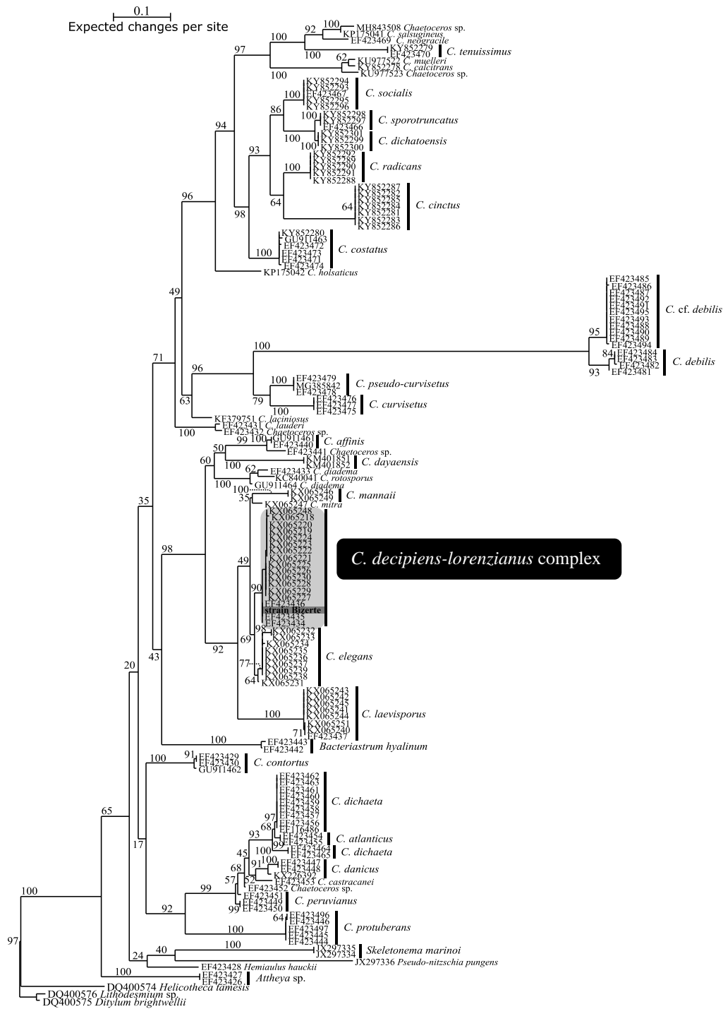
Figure 1: Maximum likelihood (ML) phylogenetic tree based on LSU rDNA sequences (148 sequences/650 characters). The tree was rooted using Lithodesmium / Ditylum as out-group
