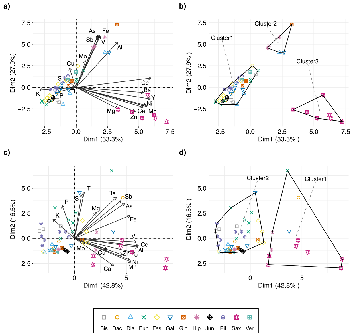
Figure 2: Biplot of the results of a primary component analysis of the elements concentrations in aerial parts (a) and roots (c) including the individuals according to their species and results of partitioning clustering (K-means) on elemental concentrations in aerial plant parts (b) and roots (d) with a Hopkins clustering tendency of respectively 0.19 and 0.20. Coloured symbols representing the 12 plant species Bis ( Biscutella laevigata ), Dac ( Dactylis glomerata ), Dia ( Dianthus sylvestris ), Eup ( Euphorbia cyparissias ), Fes ( Festuca laevigata ), Gal ( Galium corrudifolium ), Glo ( Globularia cordifolia ), Hip ( Hippocrepis comosa ), Jun ( Juniperus communis subsp. nana ), Pil ( Pilosella peleteriana ), Sax ( Saxifraga paniculata ) and Ver ( Veronica fruticans ).
