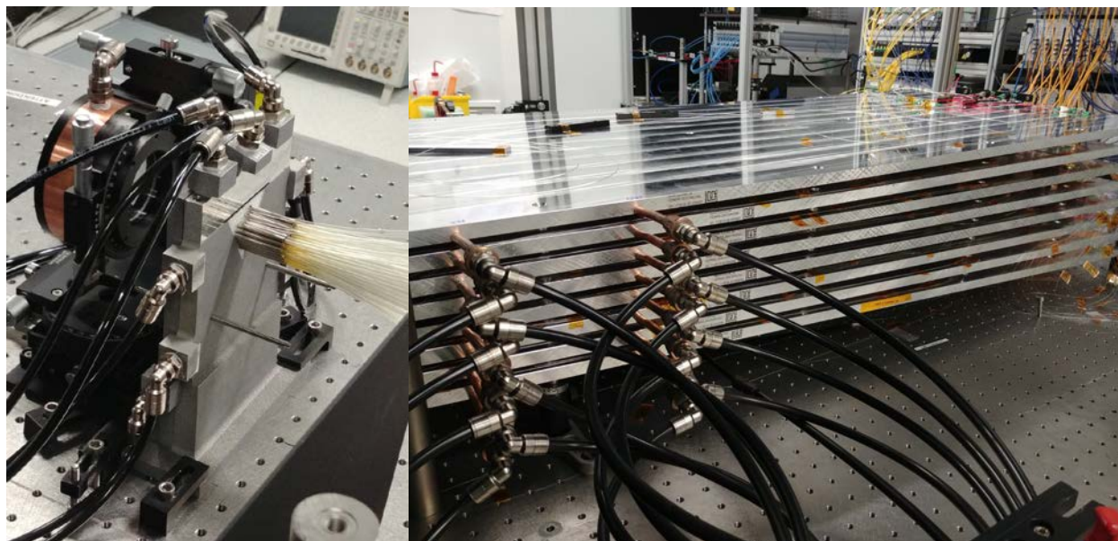
Figure 2. Water-cooled XCAN amplifiers supporting plates (right). Water-cooled 3D printed Aluminium laser head and microlens array (left).
