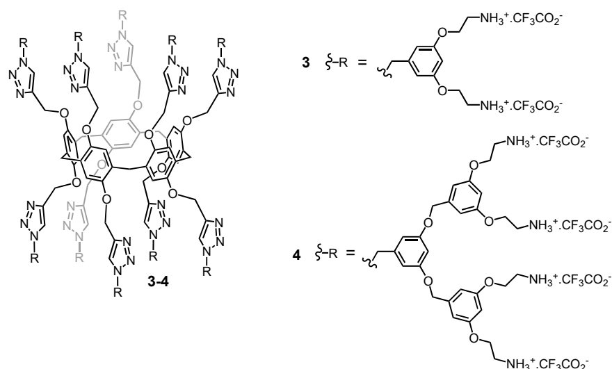
Figure 3. Dendronized pillar[5]arenes with peripheral ammonium functions (molecular weights (MW): 5787.41 ( 3 ); 11368.67 ( 4 )). These polycationic derivatives have been used as non-viral gene vectors.
