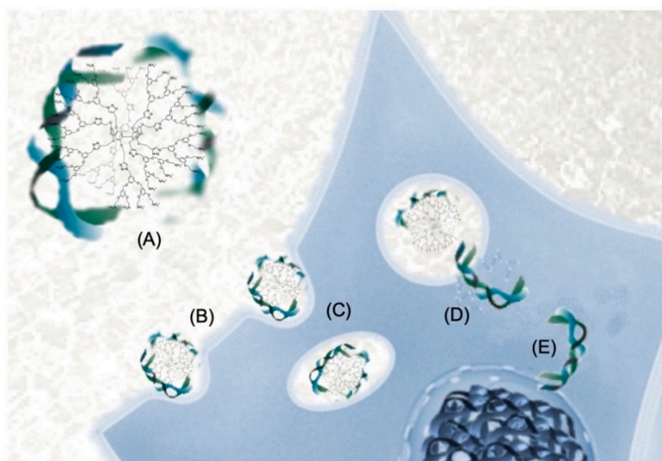
Figure 4. Schematic representation of the main step of gene delivery into a cell: (A) complexation of DNA; (B) interaction with the cellular membrane; (C) entry into the cell; (D) release into the cytosol; (E) intracellular transport into the nucleus where the DNA is expressed.
