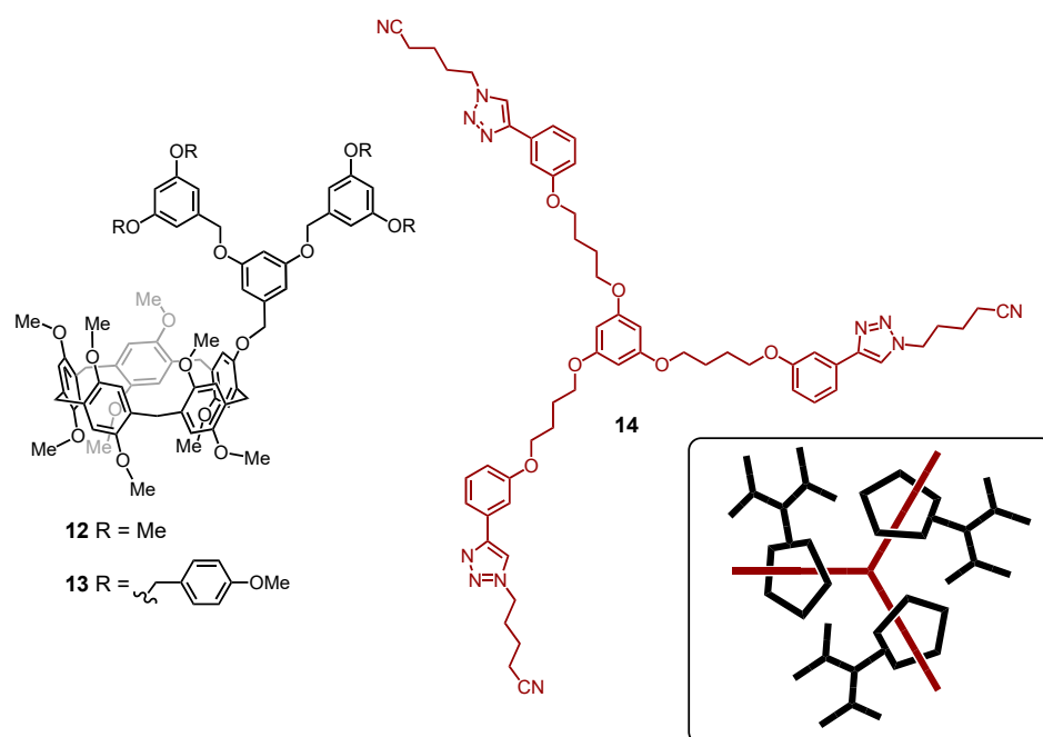
Figure 9. Dendronized pillar[5]arene derivatives 12 and 13 , and tritopic ligand 14 . The inset shows a schematic representation of the self-assembled dendrimer resulting from the binding of 14 with three pillar[5]arenes 13 (MW: 1159.34 ( 12 ); 1463.73 ( 13 )).
