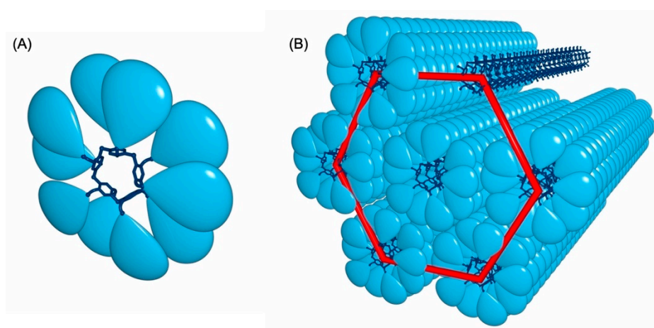
Figure 8. (A) Schematic representation of compound 11 . (B) Supramolecular arrangement of compound 11 into the hexagonal columnar phase, the dendrons have been omitted in one column (top right) to highlight the nanotubular arrangement of the pillar[5]arene cores.
