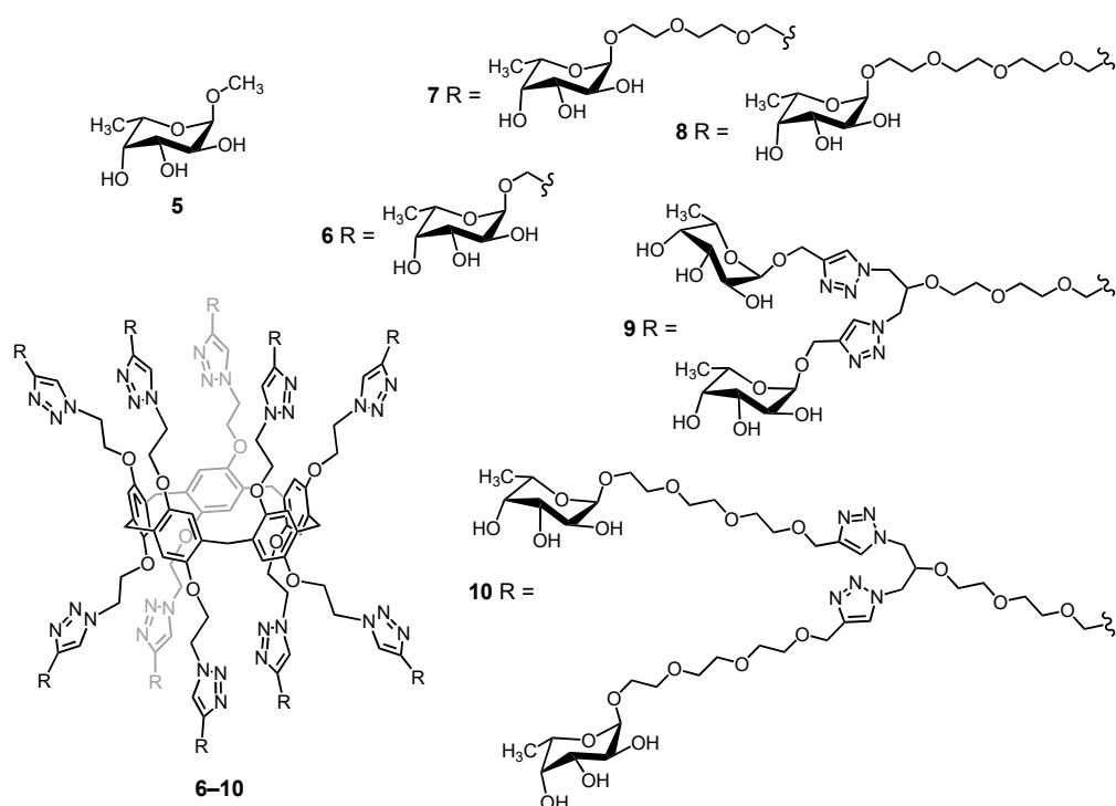
Figure 5. Model monovalent ligand 5 and glycopillar[5]arenes with 10 and 20 peripheral fucose subunits (MW: 3323.31 ( 6 ); 4204.41 ( 7 ); 4644.94 ( 8 ); 8028.18 ( 9 ); 10671.86 ( 10 )).
