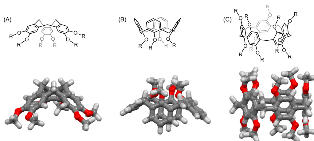
Figure 1. (A) Cyclotrimeratrylene; (B) calix[4]arene; (C) pillar[5]arene. The calculated structures of the methoxy-substituted derivatives highlight the different conformations adopted by these macrocycles: cone-shape in the case of the CTV and the calix[4]arene, and tubular in the case of the pillar[5]arene.
