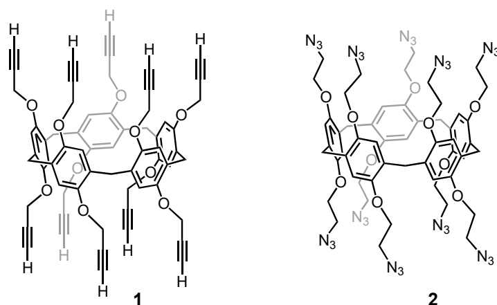
Figure 2. Typical examples of clickable pillar[5]arene derivatives used for the construction of multi-functional nanomaterials.
