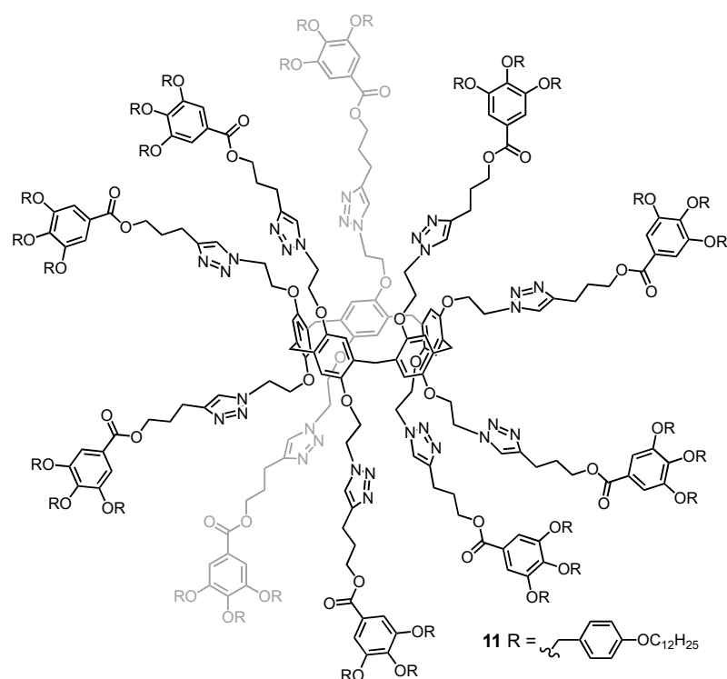
Figure 7. Dendronized pillar[5]arene 11 (MW: 11896.72).
