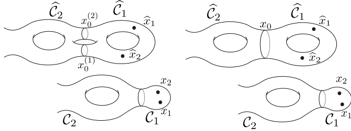
FIGURE 1. Examples of degeneracy of canonical n -covers (before colliding the zeros): on the left n = 4 and on the right n = 3 .
