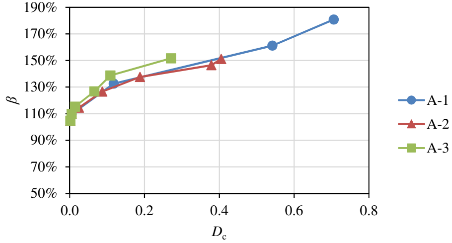
Figure 7 Variation of non-uniformity ratio \beta in MD DCB specimens as a function of D_c for three lay-ups: A-1 [\alpha/-\alpha_2/\alpha/-\alpha/\alpha_2/-\alpha]_{sym} , A-2 [\alpha/-\alpha/0/-\alpha/\alpha/0]_{anti-sym} , and A-3 [\alpha/0/-\alpha/-\alpha/0/\alpha]_{anti-sym} using the material T800/X850 (M-1)
