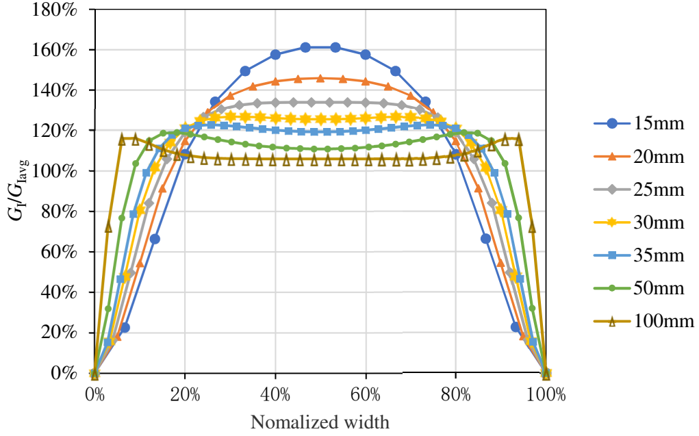
Figure 5 Width-wise distribution of G_I/G_{avg} of MD DCB specimen with different normalized widths b from T800/ X850 (M-1) having the stacking sequence [\alpha / -\alpha_2 / \alpha / -\alpha / \alpha_2 / -\alpha]_{sym} with \alpha = 30^\circ and h = 1.48 mm
