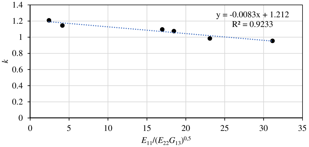
Figure 11 Linear relationship between k and \sqrt{E_{11}^2 / (E_{22}G_{13})}
