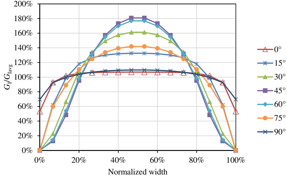
Figure 6 Width-wise distribution of G_I/G_{Iavg} of MD DCB specimen with different fiber orientation angle \alpha from T800/X850 (M-1) having the stacking sequence [\alpha/-\alpha_2/\alpha/-\alpha/\alpha_2/-\alpha]_{sym} with b = 15 mm, h = 1.48 mm
