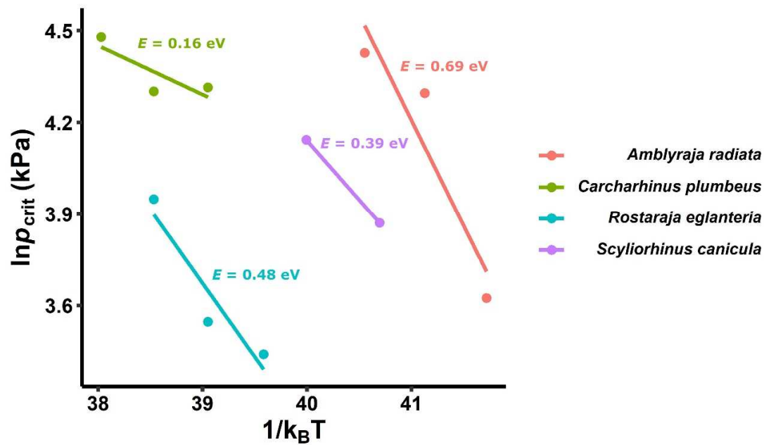
Fig. 5. Temperature sensitivity of critical oxygen tension ( p_{crit} ) of four elasmobranch species. The natural logarithm of p_{crit} (kPa) is plotted against the inverse of temperature ( ^{\circ}\text{Kelvin} ) multiplied by the Boltzmann constant. The slope of this line is the temperature sensitivity ( E , in eV). Available data from the literature were collected for the thorny skate, Amblyraja radiata (Schwieterman et al., 2019b), sandbar shark, Carcharhinus plumbeus (Crear et al., 2019), clearnose skate, Rostaraja eglanteria (Schwieterman et al., 2019b), and small-spotted catshark, Scyliorhinus canicula (Butler and Taylor, 1975).
