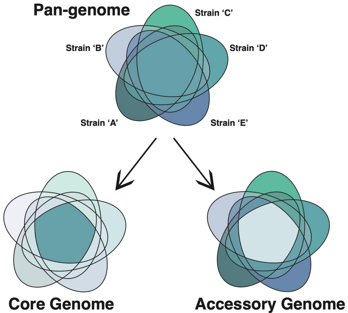
Figure 2. Pan-genome schematic. The pan-genome consists of all genes found in a given species. This is comprised of a 'core' genome (genes found in all strains) and an 'accessory' genome (genes found in a single strain (i.e. strain specific) or a subset of strains (i.e. strain select)).
