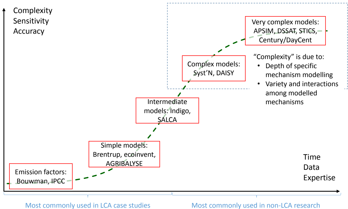
76 77 Fig. 1. Modelling continuum for estimation of N emissions in the French LCA context
