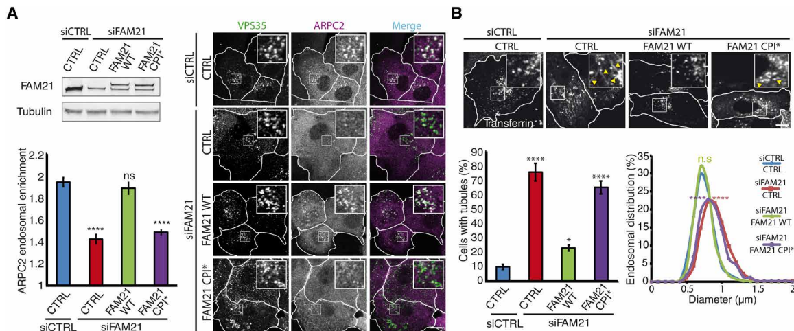
Fig. 4. Deficient uncapping alters endosomal structures. (A) Endogenous FAM21 was depleted from MCF10A control cells or stable MCF10A lines expressing GFP-FAM21 WT or CPI* using siRNAs. Endosomal branched actin structures were estimated by the overlap of ARP2C2 (Arp2/3) with VPS35 (retromer). Scale bar, 10 \mu m. (B) Endosomes were loaded at steady state with fluorescent transferrin. Endosomal size and the presence of tubules (arrowheads) were estimated from live-cell confocal imaging.
