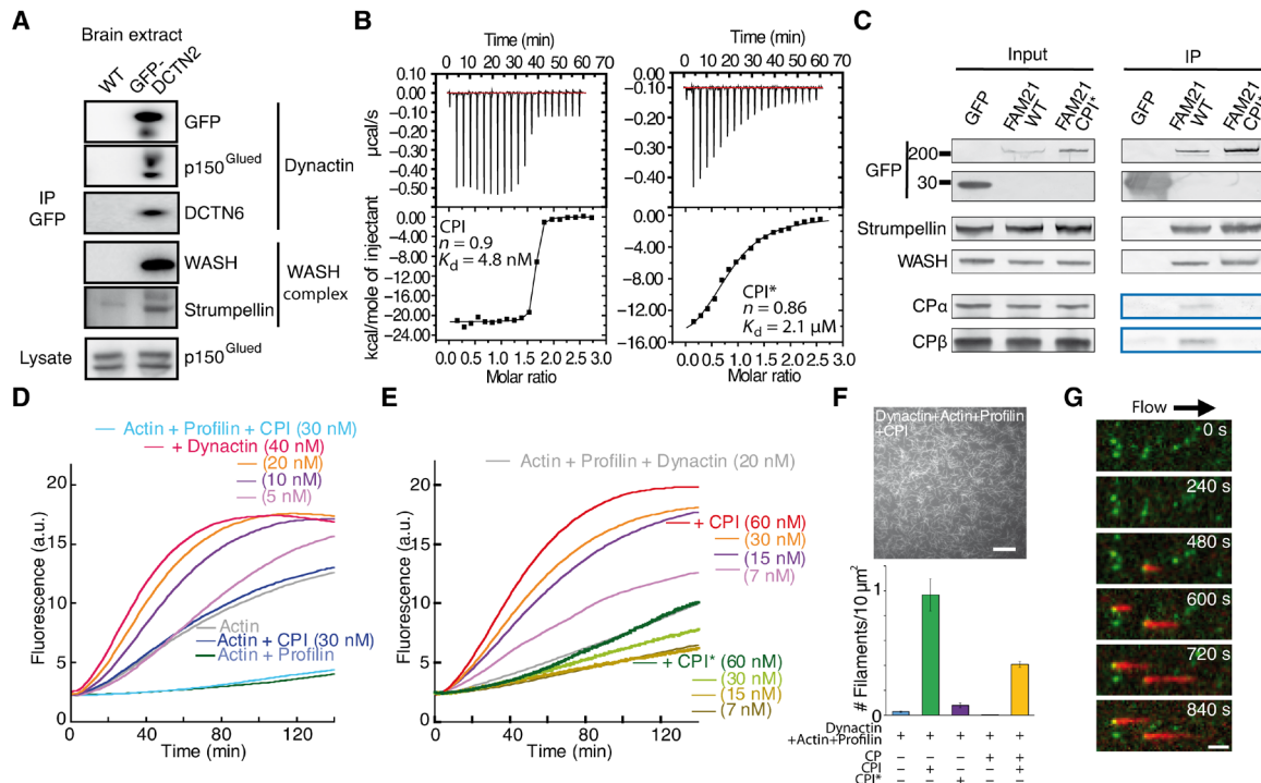
Fig. 1. The CPI motif of FAM21 induces actin elongation from dynactin. (A) The WASH complex coprecipitates with GFP-tagged dynactin (GFP-DCTN2) from the brain of a transgenic mouse. (B) Isothermal calorimetry of the interaction between CP and WT CPI or CPI*, a variant containing three point mutations. Curve fits indicate the stoichiometry of interaction ( n ) and K_d (dissociation constant). (C) Stable expression of GFP-FAM21 CPI* in MCF10A cells reconstitutes a WASH complex that does not recruit CP. (D and E) Pyrene-actin polymerization assays. Conditions: 2.0 \mu\text{M} actin (5% labeled), 8 \mu\text{M} profilin, native dynactin, CPI, or CPI*. a.u., arbitrary units. (F) TIRF imaging of filaments elongated from surface-anchored dynactin in the presence of CPI. Observation 10 min after having introduced 1 \mu\text{M} labeled actin, 8.2 \mu\text{M} profilin, 0 or 2 \mu\text{M} CP, and 0 or 2.7 \mu\text{M} CPI in F-buffer. Scale bar, 20 \mu\text{m} . (G) Time-lapse images of actin filaments growing under flow from GFP-DCTN3-labeled dynactin (green). Conditions: 1 \mu\text{M} actin (15% labeled, red), 1 \mu\text{M} profilin, 50 nM CPI. Scale bar, 3 \mu\text{m} .
