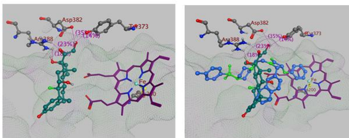
Figure 5. The best pose of dexamethasone with x-ray crystal structures (PDB code: 2NSI) in the active site of iNOS; and the residues of the active site involved in ligand binding (left). Superimposition of 4b (blue) and dexamethasone (green) within the enzyme binding site (right).
