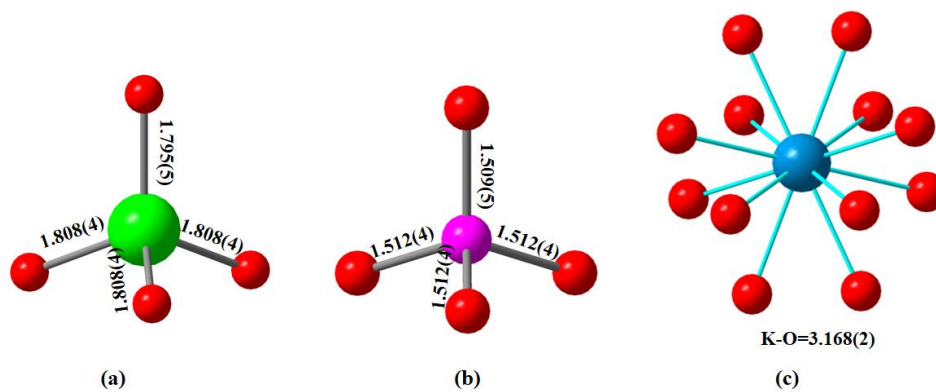
Figure 8. Polyhedrons representing the geometries of coordination environments of (a) M, (b) P and (c) K in the \text{KMgAl}(\text{PO}_4)_2 structure.
