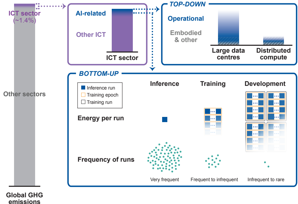
Figure 2: Compute-related global greenhouse gas (GHG) emissions impacts of machine learning (ML). The information and communications technology (ICT) sector accounts for around 1.4% of GHG emissions today, of which ML likely accounts for a small but unknown share (indicated by shading). Compute-related impacts of ML can be assessed from both top-down and bottom-up perspectives. Top-down: The majority of ML-related GHG emissions likely come from compute loads in large data centers, with a smaller share from distributed compute (e.g., personal computers, smartphones); these GHG emissions result from both operational energy use from computation and from other phases of the hardware life cycle (including embodied emissions). Bottom-up: The amount of energy needed for an ML model throughout different stages of the model life cycle differs based on problem setting and usage patterns.
