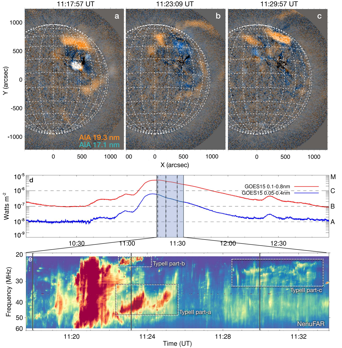
Figure 1. (a, b, c) SDO 17.1 nm (blue) and 19.3 nm (orange) running ratio observations of the eruption from AR 12736. An EUV wave is seen propagating both on-disk and off-limb, visible as enhanced emission in 19.3 nm (orange regions). (d) Geostationary Operational Environmental Satellite (GOES) light curve of the C4.8 flare. The shaded region indicates the time interval of the dynamic spectrum and the vertical dashed lines are the times of the AIA images. (e) NenuFAR observations showing a summary of radio bursts taking place during the flare from 11:17:30–11:33:30 UT. The type II radio burst starts in the NenuFAR frequency range at 11:22 UT and we have labeled three different parts (type II parts-a, b, and c), which we examine separately. The solid vertical lines on the dynamic spectrum indicate the times of the AIA images.
