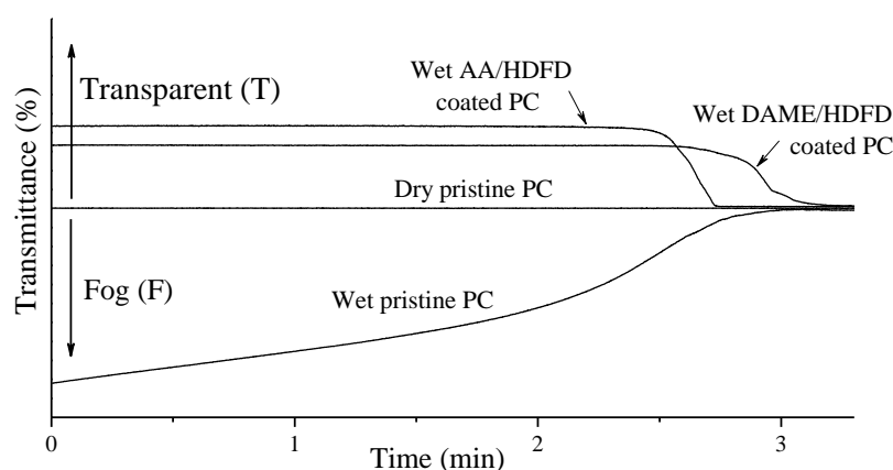
Figure 5. Light transmission ( \lambda = 550 nm) over time through the dry, wet pristine and coated PC : p-DAME-co-HDFD, p-AA-co-HDFD exposed 1 min to the water vapor ([HDFD] = 20 %, P = 10 W, f = 6 kHz, d.c. = 10 %, t = 10 min).
