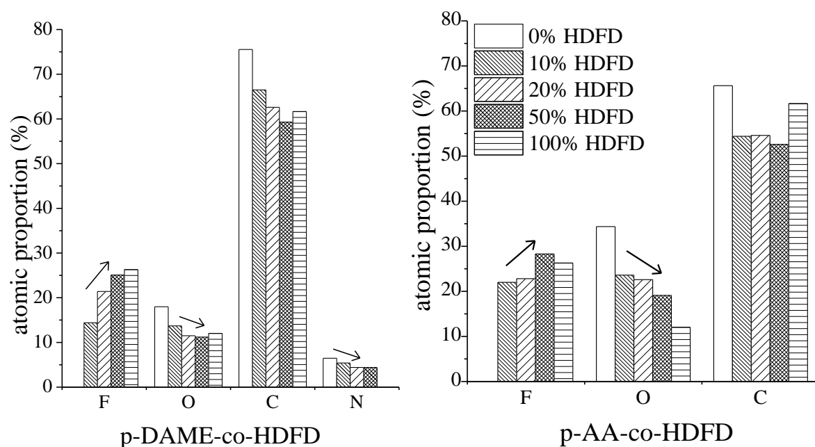
Figure 2. Dependence of the atomic F, C, O, N percentages (XPS data) in (co)polymers on the HDFD concentration in the plasma phase ( P = 10 \text{ W} , f = 6 \text{ kHz} , d.c. = 10 \% , t = 10 \text{ min} ).
