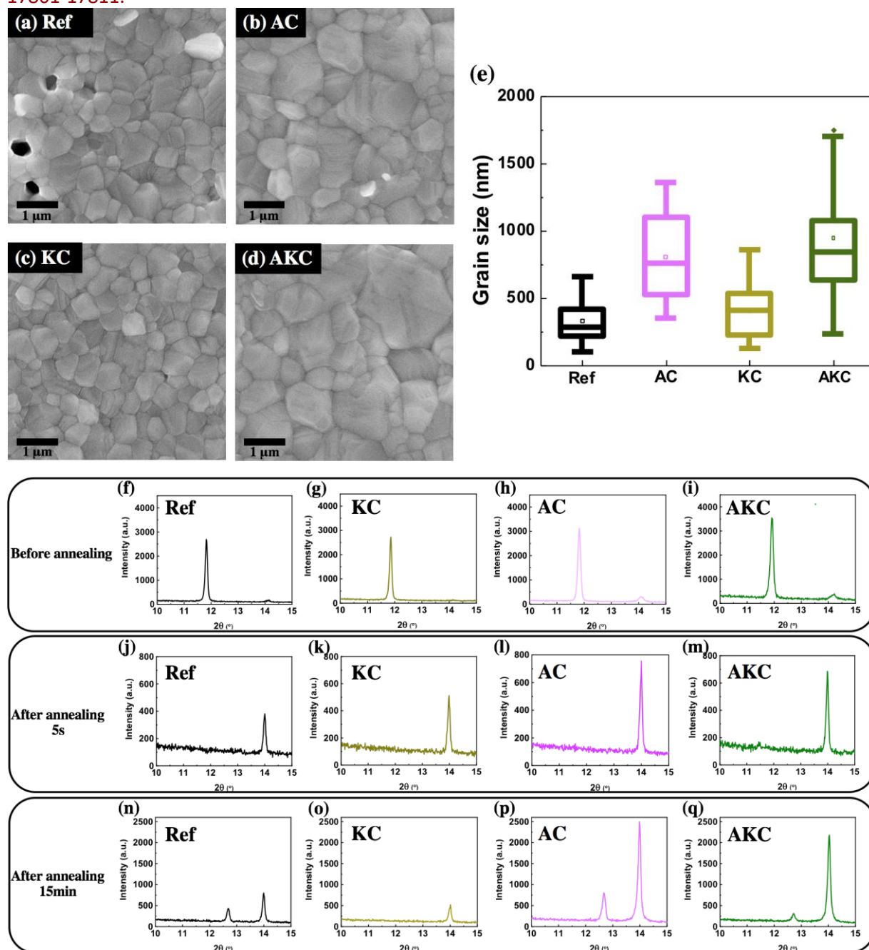
Figure 2. (a-d) SEM top-views of the \text{Cs}_{0.1}\text{FA}_{0.9}\text{PbI}_3 films. (e) Effect of chloride additives on the grain size. (f-m) Effect of chloride additives on the XRD pattern of the films produced by spin-coating, before annealing (f-i), after 5 s of annealing (j-m) and after (n-q) full annealing.
