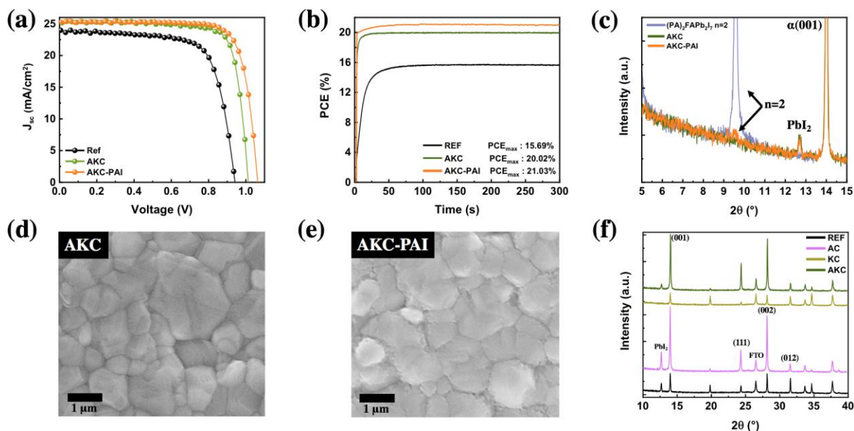
Figure 1. Effects of Cs_{0.1}FA_{0.9}PbI_3 engineering and capping layer on (a) the reverse scan J - V curves, (b) steady-state PCE at the maximum power point. (c) XRD patterns of the pristine and PAI treated AKC layer and of a 2D (PA)_2FAPb_2I_7 film. SEM layer top view before (d) and after (e) PAI treatment. (f) Effect of chloride additives on the XRD patterns.
