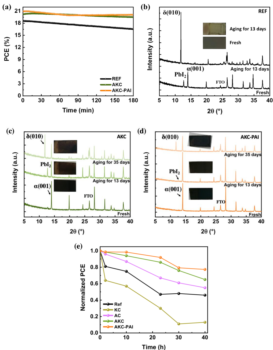
Figure 5: (a) Tracking of the Ref, AKC and AKC-PAI cells at their maximum power point; (b-d) XRD patterns of the (b) Ref, (c) AKC and (d) AKC-PAI layers under ambient condition (20°C, 55±10% RH). The insets are layers pictures. (e) Normalized PCE evolution of cells stored under ambient condition and very high humidity (RH≥90%).
