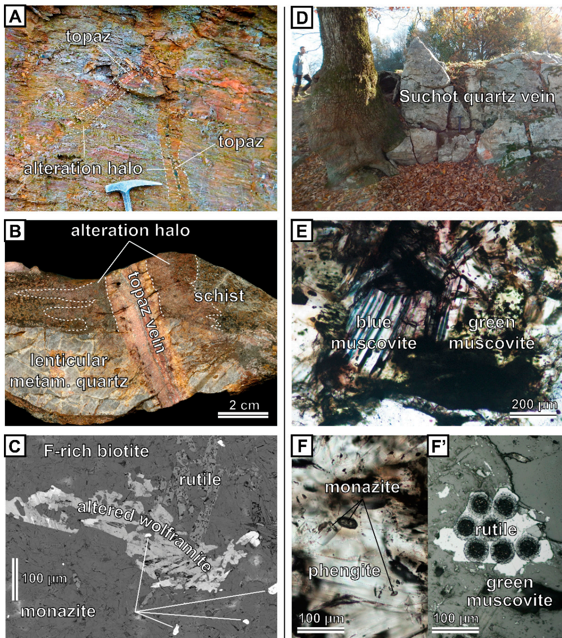
Figure 2. Alteration haloes and mineral textures from the topaz (A–C) and Suchot (D–F) veins. (A): Outcrop image of topaz veins and their alteration halos. Colors are saturated for better clarity. (B): Photograph of topaz vein sample crosscutting the metamorphic foliation. Alteration halo is well marked in the schist. (C): Backscattered electron image of altered wolframite b and associated monazite in the alteration halo of the topaz veins. Matrix of the alteration is mostly composed of F-rich brown micas (D): Outcrop photograph depicting the metric-sized Suchot vein. (E): In the selvage of the Suchot vein, metamorphic minerals are entirely replaced by hydrothermal quartz and two generations of micas: green and pale-blue colored muscovite crystals. Photomicrograph is in Plane-Polarized Light (PPL). (F): Blue muscovite crystals display numerous inclusions of monazite while rutile inclusions are lacking (PPL). (F'): Reflected light image of rutile crystal included in green muscovite. Conversely to blue muscovite, monazite inclusion is scarce in this type of micas.
