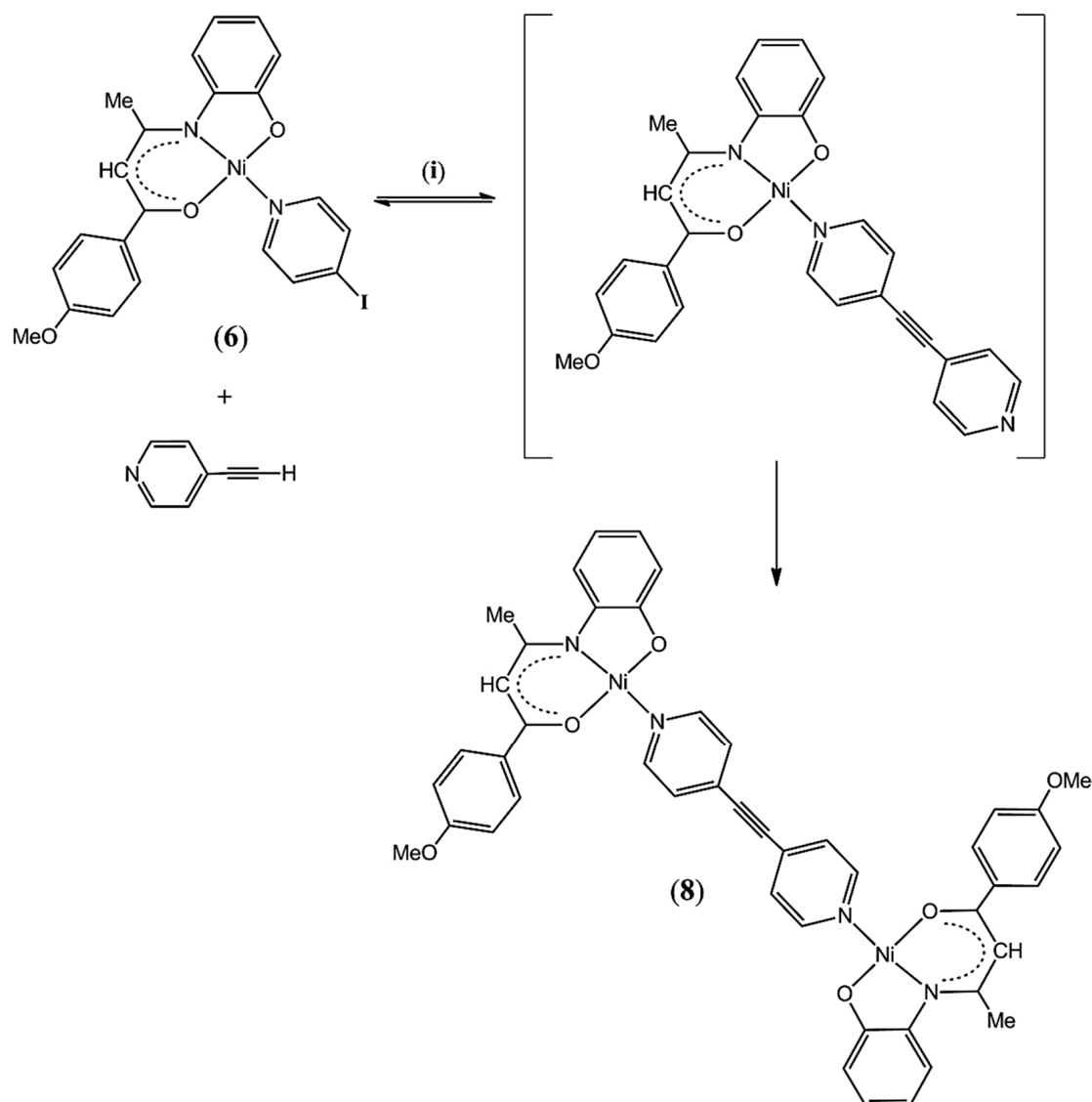
Scheme 2. Formation of the binuclear complex 8; (i) = trans -PdCl 2 (PPh 3 ) 2 , CuI, TEA:THF (1:5, v:v ), 12 h at 20 °C.
