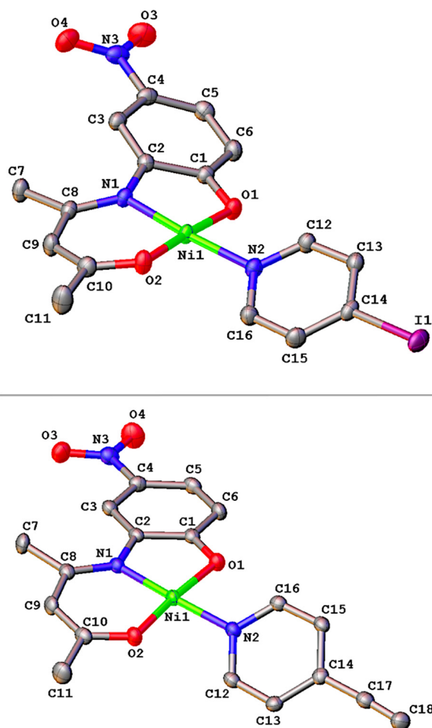
Figure 1. Molecular structures of complexes 4 (top) and 5 (bottom), with labelling scheme for selected atoms. Hydrogens have been omitted for clarity. Thermal ellipsoids are drawn at the 50% probability level.
