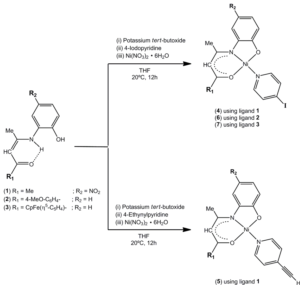
Scheme 1. Synthesis of complexes 4–7.
