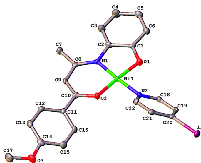
Figure 2. Molecular structure of complex 6 with labelling scheme for selected atoms. Hydrogens have been omitted for clarity. Thermal ellipsoids are drawn at the 50% probability level.
