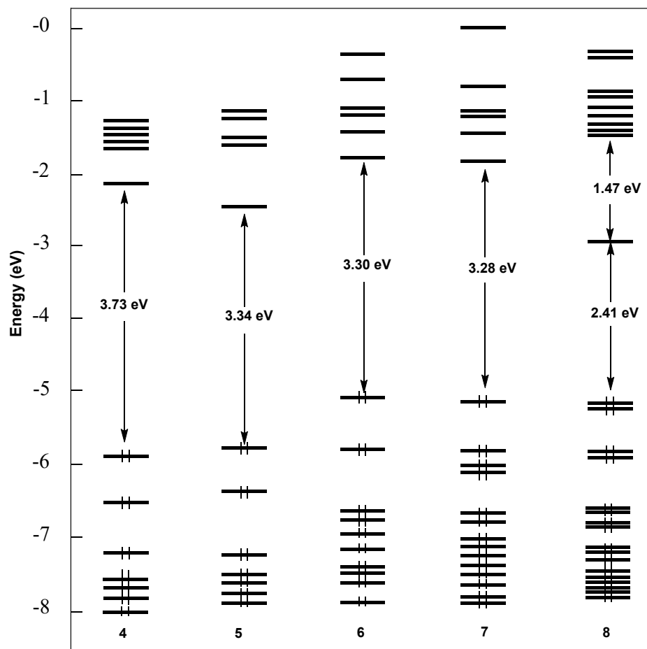
Figure 5. The MO energy level ordering of the five investigated complexes.
