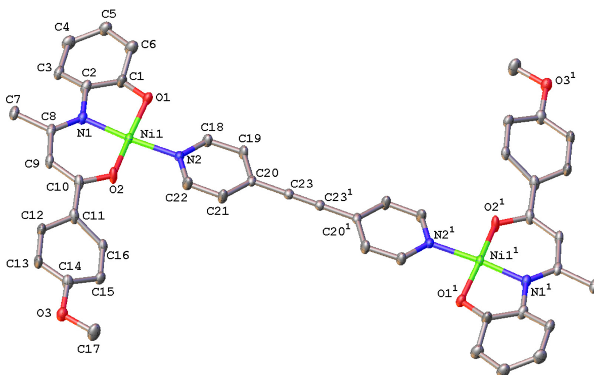
Figure 3. Molecular structure of complex 8 (molecule A) with labelling scheme for selected atoms. Hydrogens have been omitted for clarity. Thermal ellipsoids are drawn at the 40% probability level. Half unit of molecule was generated by symmetry operations -x, -y, -z .
