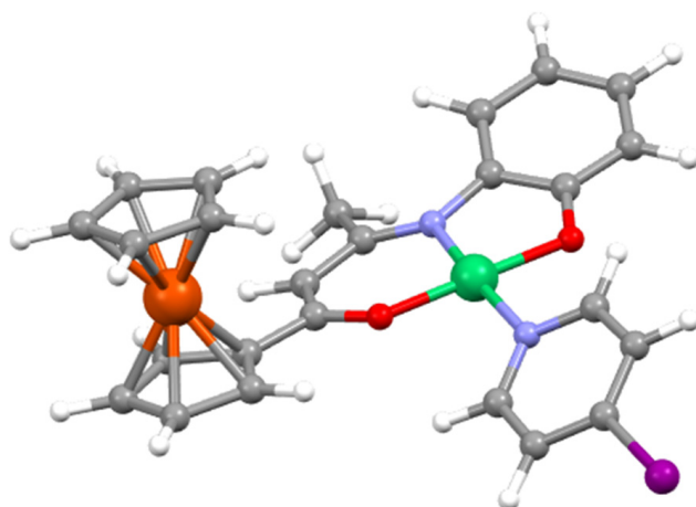
Figure 4. The DFT-optimized structure of complex 7.
