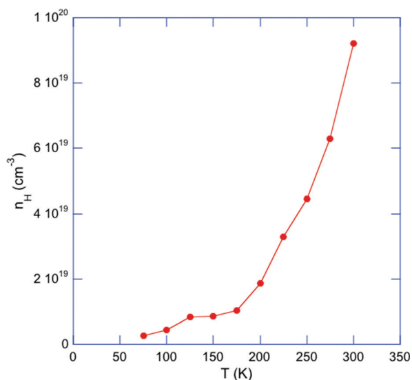
Fig. 8 Temperature dependence of the electron concentration n_{\text{H}} for \text{Tl}_{0.6}\text{Mo}_3\text{S}_5 . The solid line is a guide to the eye.
