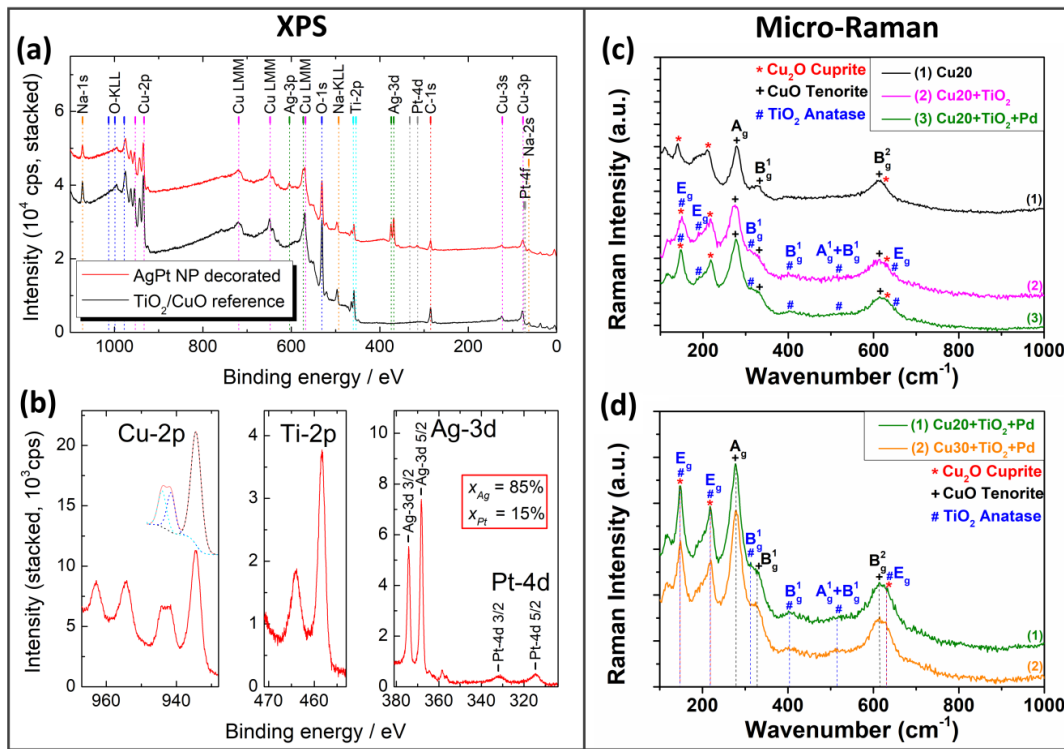
Fig. 3. X-ray photoelectron spectra (XPS) of: (a) a AgPt/TiO 2 /CuO/Cu 2 O (red line) nanocomposite and an undecorated TiO 2 /CuO/Cu 2 O thin film (black line); (b) spectra at higher resolution for Cu-2p and Ti-2p lines as well as spectra for Ag-3d and Pt-4d lines. Micro-Raman spectra for: (c) the surface functionalized TiO 2 /CuO/Cu 2 O and Pd/TiO 2 /CuO/Cu 2 O samples with CuO/Cu 2 O thickness of 20 nm (Cu 20 ) after being thermally treated at 420°C for 30 min in ambient; (d) Pd/TiO 2 /CuO/Cu 2 O with CuO/Cu 2 O thicknesses of 20 nm (Cu 20 ) and 30 nm (Cu 30 ), respectively.
