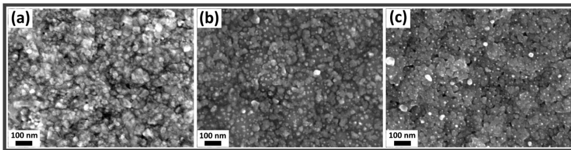
Fig. 2. Higher magnification of SEM images of interconnected nano-crystallite TiO 2 /CuO/Cu 2 O covered with: (a) Pd nanoparticles, Cu20 set samples; (b) Ag nanoparticles, Cu60 set samples; (c) AgPt nanoparticles, Cu60 set samples, nanoclusters of 5-15 nm in diameter.
