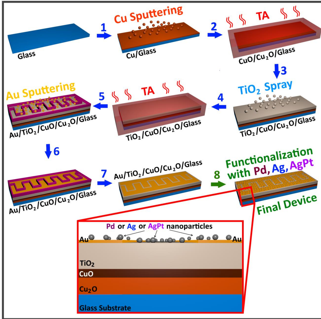
Fig. 1. (a) The technological flowchart for the manufacture of sensor device structures based on nanostructured layered films consisting of Pd, Ag or AgPt NPs on top of TiO 2 /CuO/Cu 2 O (Final device structure). Cross-section view of a device based on Pd, Ag or AgPt NPs on top of the TiO 2 /CuO/Cu 2 O -based sensor in insert from (a).
