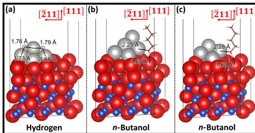
Fig. 9. Adsorption of: (a) H 2 , and (b and c) n -C 4 H 9 OH on the TiO 2 (111)/CuO( \bar{1}\bar{1}\bar{1} )/Cu 2 O(111) heterostructure decorated with the Pd 7 , Ag 7 and Ag 6 Pt clusters, respectively. Interatomic distances are shown and crystallographic directions are indicated with respect to the Cu 2 O(111) substrate. The ternary heterojunctions functionalised using the Pd 7 , Ag 7 or Ag 6 Pt nanoparticles are displayed using the space-filling representation, whereas the adsorbates are shown using the stick representation. O atoms are in red, H atoms are in white, C atoms are in brown, Cu atoms are in dark blue, Ti atoms are in light blue and Pd, Ag and Pt atoms are in grey.
