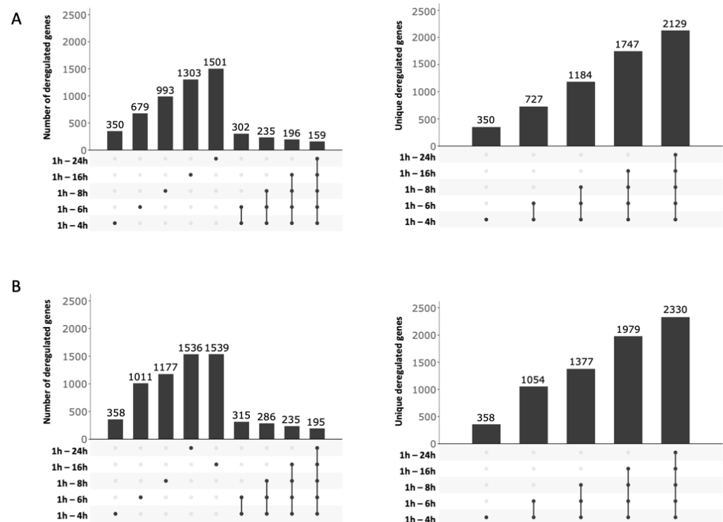
Figure 5. Evolution of deregulated genes from W37 (A) and D37 (B) strains after the temperature shift. The left panels show the number of differentially expressed genes at each time point (see Table S6) and the number of common genes among indicated time intervals (illustrated by solid black points, linked by black lines). The right panel shows the increasing number of unique genes that are differentially expressed at a minimum of one time point after the temperature shift. Number of deregulated genes ( |FC| \geq 2 , p -value \leq 0.01 ).
