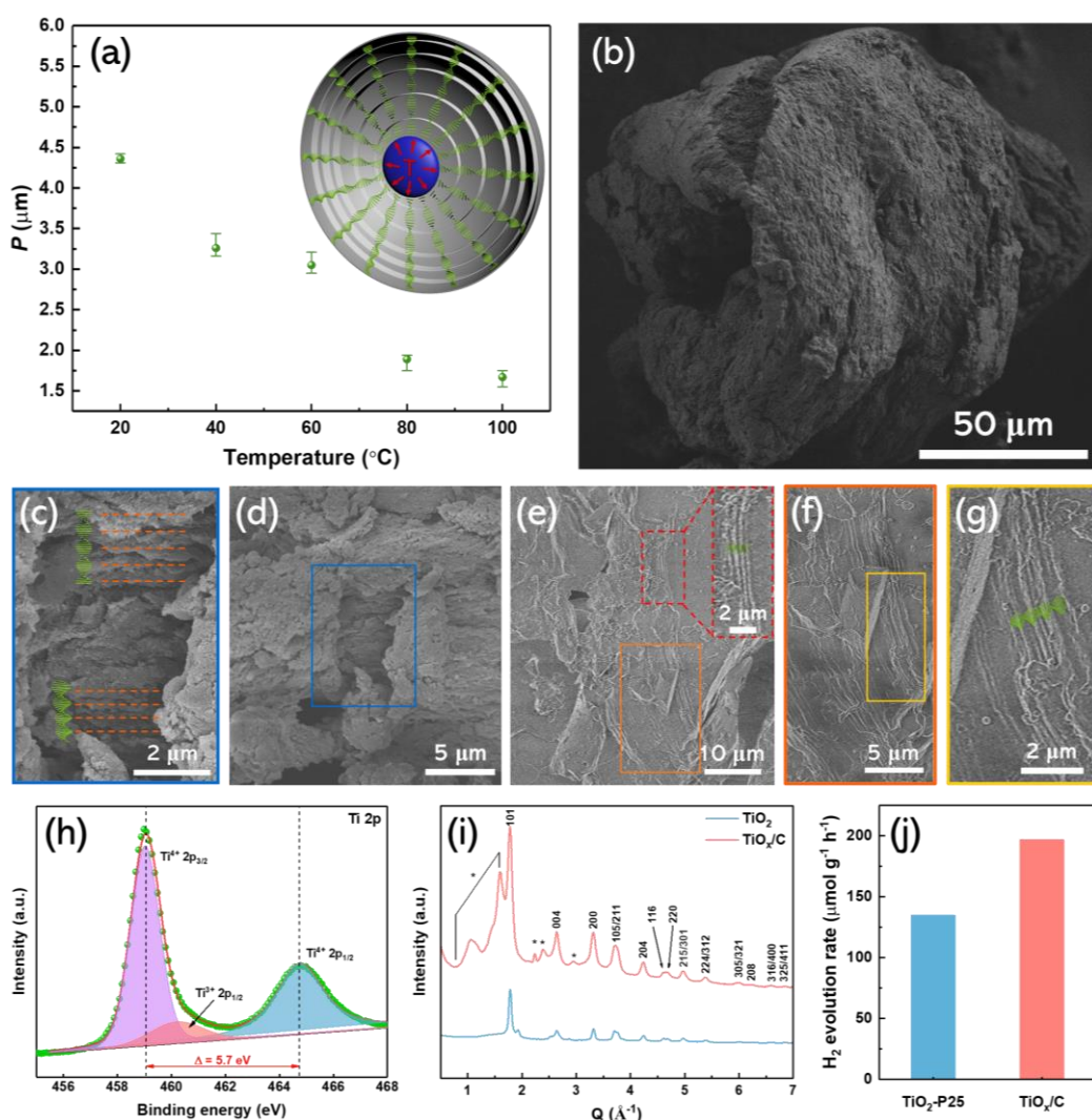
Figure 5. (a) The effect of temperature on P . The inset is a 3D schematic diagram of P compressed at higher temperature. (b) SEM image of \text{TiO}_2/\text{C} microsphere with wrinkles on the surface and a hole in the centre. (c-g) Cross-section SEM images of microspheres showing Ch nematic structures with periodic lamellar bands. (h) XPS spectrum of Ti 2p. (i) WAXS patterns of \text{TiO}_2/\text{C} microspheres. (j) Hydrogen generation constant rate of \text{TiO}_2/\text{C} microspheres and commercial \text{TiO}_2\text{-P25} .
