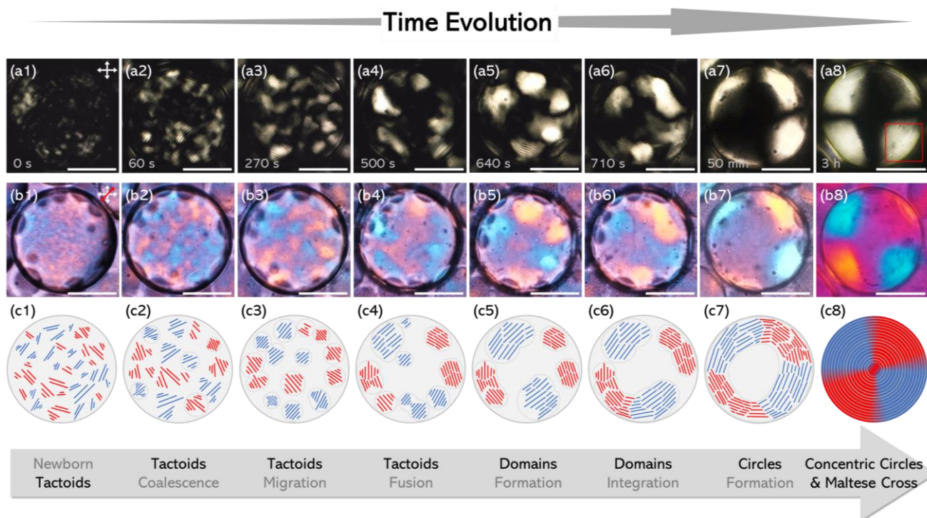
Figure 3. Typical POM images of time-series snapshots of TAA/CNC 6% microdroplet without (a1-a8) and under lambda retardation plate (b1-b8) (scale bar = 50 μm). Note that (a8) and (b8) was captured by using high magnification camera once equilibrium was reached. (c1-c8) Corresponding cartoon depiction of the microdroplet transforms from newborn tactoids to symmetrical concentric circles with Maltese cross structure.
