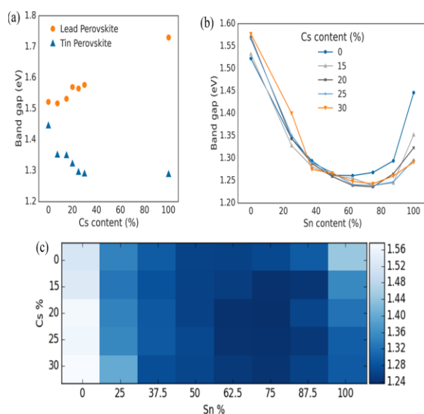
Figure 3. (a) Optical band gap of lead- and tin-based perovskites FA_{1-x}Cs_xMI_3 ( M = Sn, Pb ) as a function of cesium content. (b) Band gap of five series of tin-lead mixed perovskites, corresponding to cesium fractions of 0, 15, 20, 25, and 30%. (c) 2-dimensional map of band gap (in eV) across the formamidinium-cesium and tin-lead compositional space studied.
