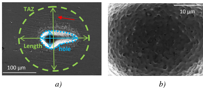
FIGURE 1. Laser impact on PEEK ( P = 5 \text{ W} , \nu = 50 \text{ kHz} ) a) 1 shot (x400), b) 2 shots (x3000)
