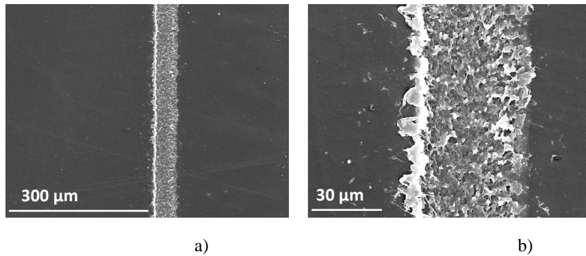
FIGURE 2. SEM pictures (a) x200; b) x1000) of etched lines ( P = 2 \text{ W} , \nu = 100 \text{ kHz} and d = 5 \text{ }\mu\text{m} )
