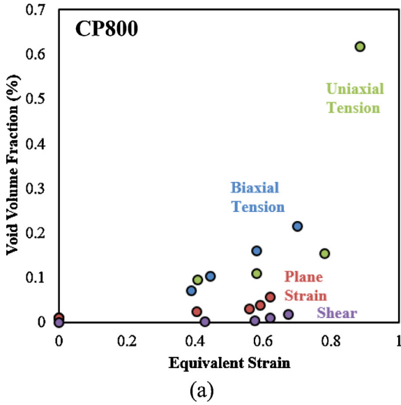
Fig. 20. Void volume fraction versus equivalent strain for (a) CP800 and (b) DP780.
