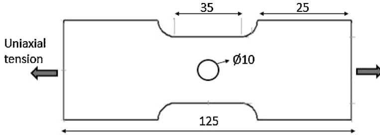
Fig. 2. Specimen geometry used for the DP780 hole tension test. All units are in mm.
