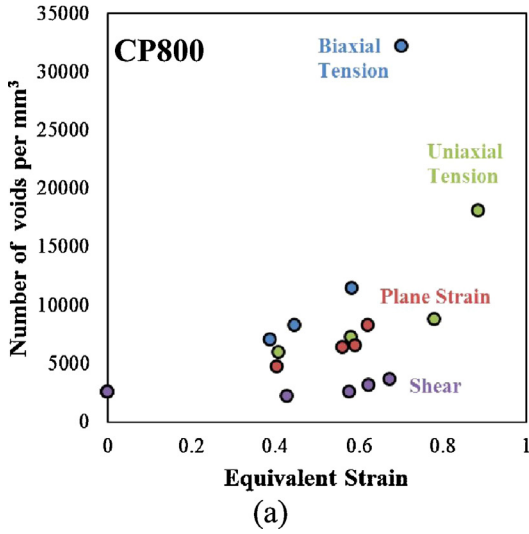
Fig. 19. Evolution of average void density with respect to equivalent strain for (a) CP800 and (b) DP780 steels.
