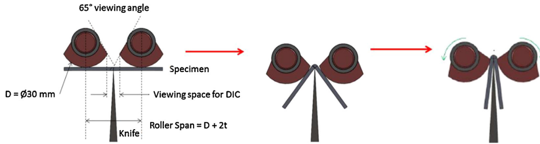
Fig. 3. Concept of Cheong et al. [46] for the tight radius v-bend process.
