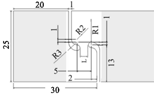
Fig. 4. Shear specimen geometry of Peirs et al. [48]. Gripped region is shaded.
