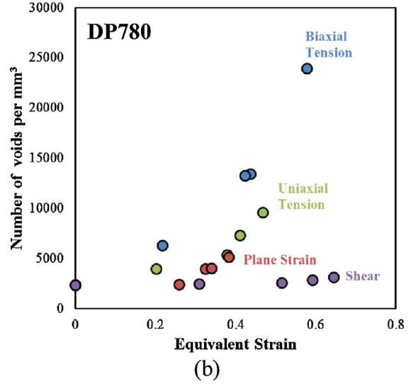
Fig. 19. Evolution of average void density with respect to equivalent strain for (a) CP800 and (b) DP780 steels.
