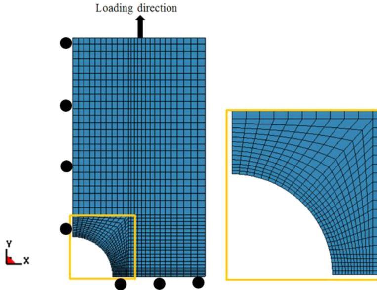
Fig. 13. Hole tension finite element mesh.
