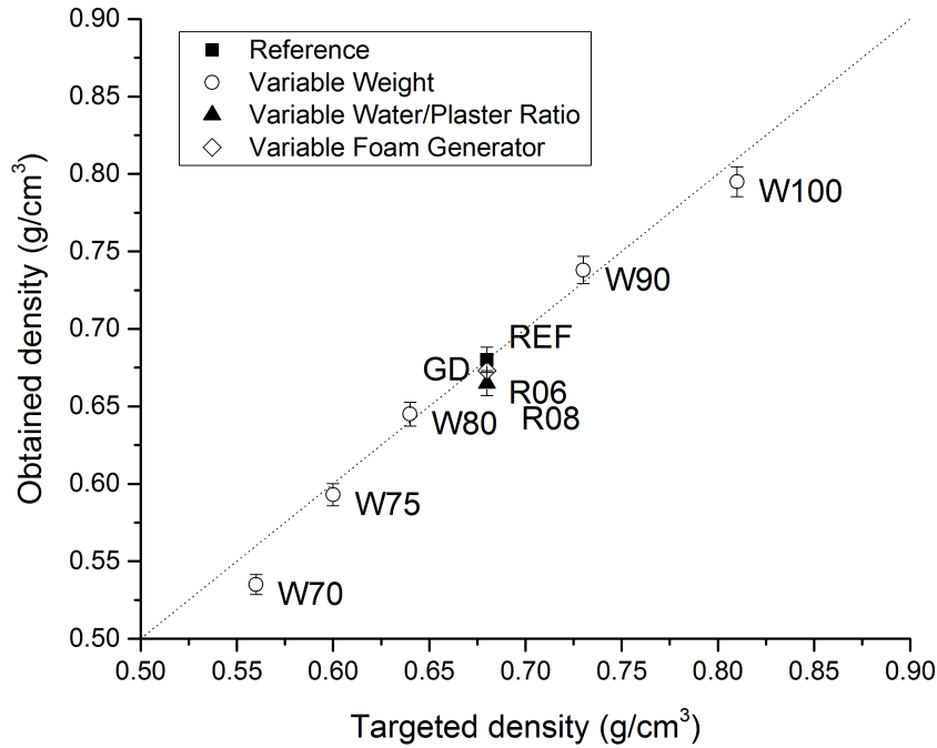
Figure 8: Obtained vs targeted density for our 9 samples. The error bar corresponds to the density measurement uncertainty mostly due to difficulties in volume measurements. The dotted line corresponds to the f(x)=x function
