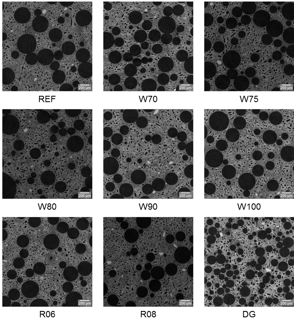
Figure 2: Slice of tomography scan with a voxel size of 2 μm for the 9 foamed gypsum formulations
