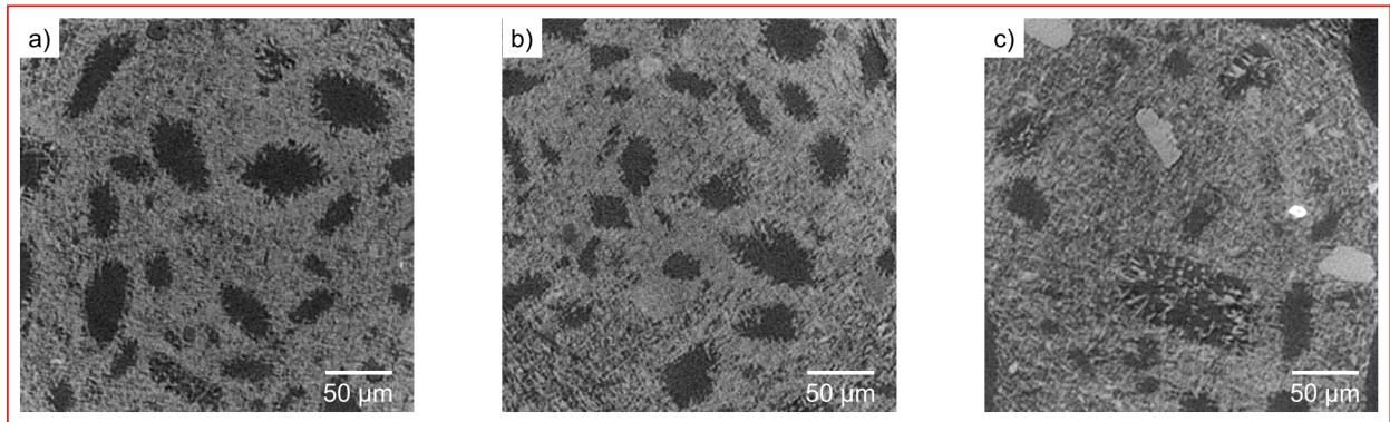
Figure 9: Slice of tomography scan with a voxel size of 0.3 μm for a) R06 (W/P = 0.6) b) REF (W/P = 0.7) c) R08 (W/P = 0.8)
