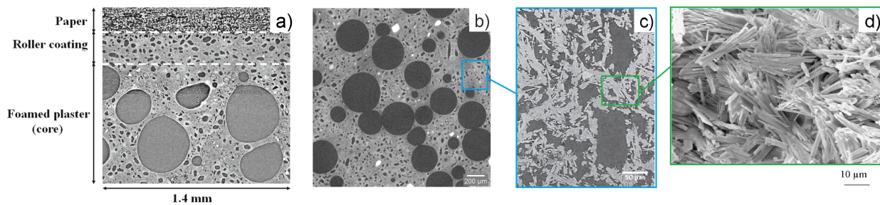
Figure 1: a) lightweight plasterboard structure: paper, roller coating and foamed plaster [9] b) macroporosity of foamed gypsum (large spherical pores) on a X-ray tomography scan with a 2\ \mu\text{m} voxel size c) mesoporosity due to hemihydrate dissolution on a tomography scan [10] d) SEM image of microporosity between entangled gypsum crystals [3]
