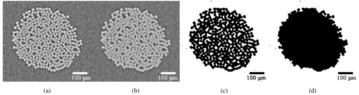
Figure 1: (a) Image of a single yarn cross-section obtained with X-ray microtomography. (b) Median filter applied to the first image. (c) Binarization of the cross-section with an adapted threshold. (d) A function "fill holes" is applied to fulfil every blank hole between the binarized fibres.
