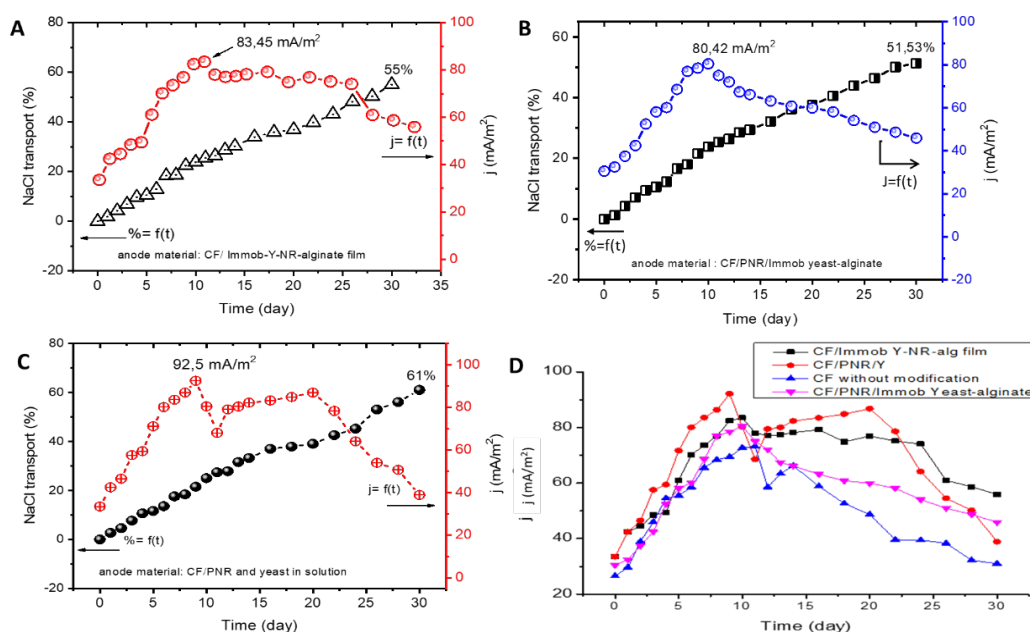
Fig. 8. The evolution of current density and % of NaCl transport generated from MDC using bio-devices modification: (a) CF/Immob Y-NR; (b) CF/PNR-Immob Y; (c) CF/PNR; (d) Summary of all MDC experiment parts.
