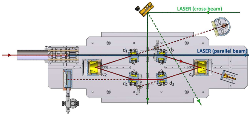
Figure 1: Schematics of the Mini-Ring
